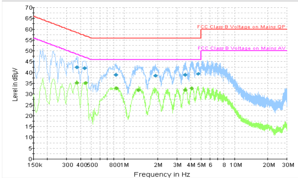
Fig.7 Conducted Emission
