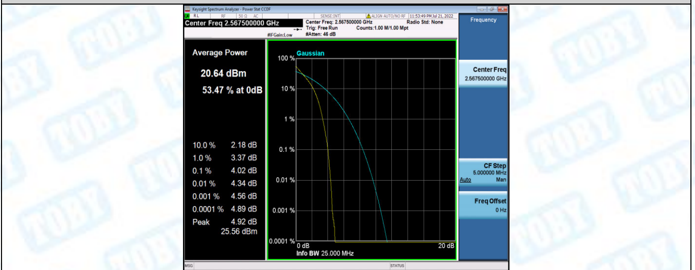
Band7-5MHz-16QAM-20775-1RB#0
