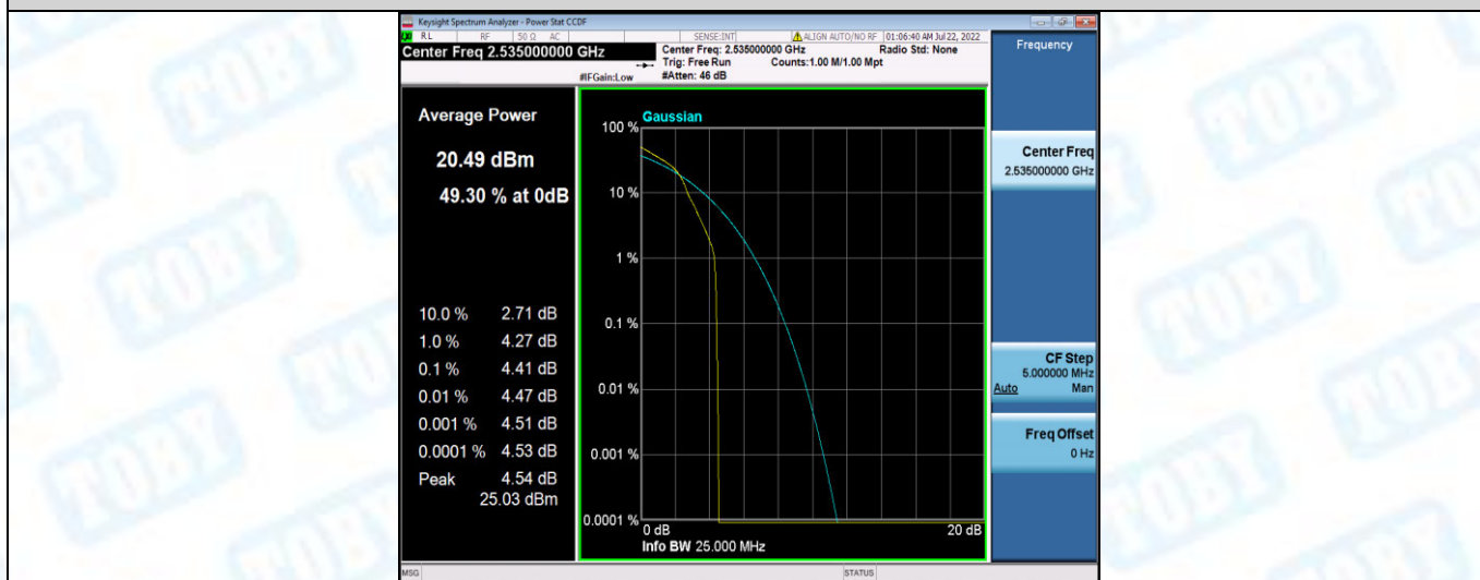
Band7-20MHz-16QAM-21100-100RB#0
