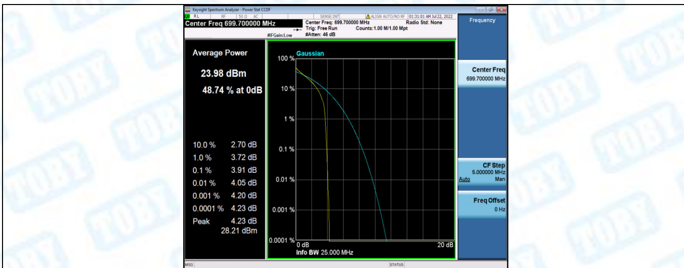
Band12-1.4MHz-QPSK-23017-6RB#0
