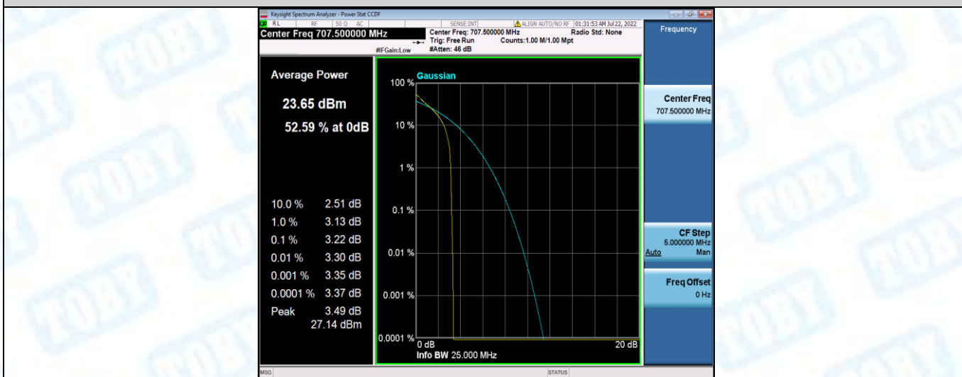
Band12-1.4MHz-QPSK-23095-6RB#0
