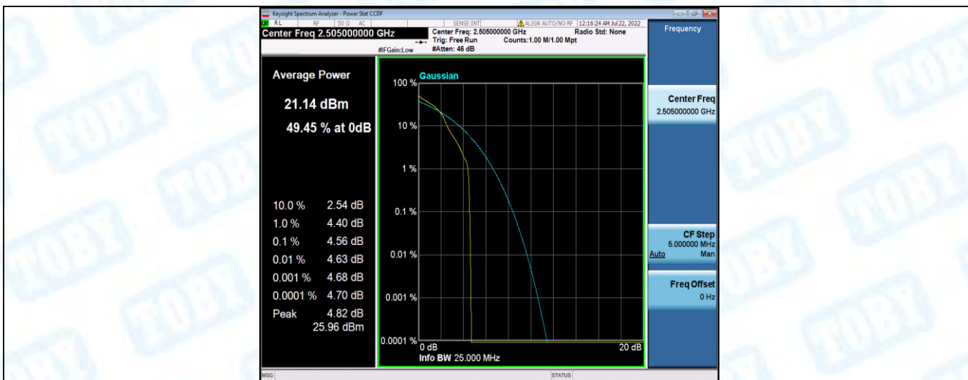
Band7-10MHz-16QAM-20800-50RB#0
