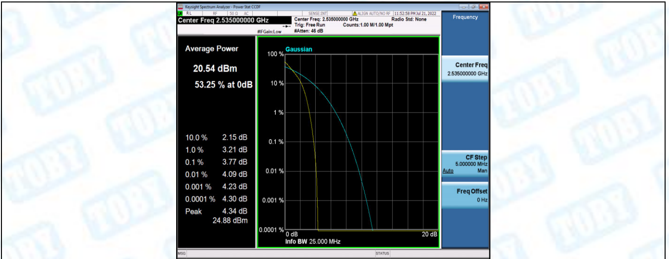
Band7-5MHz-QPSK-21425-1RB#0
