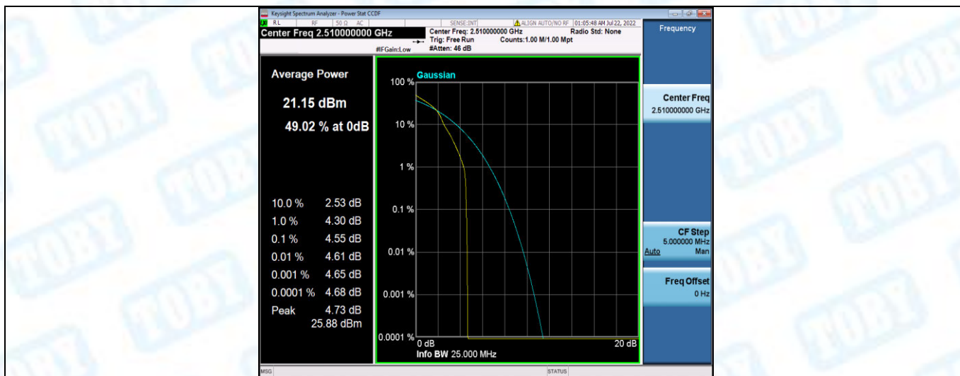
Band7-20MHz-16QAM-20850-100RB#0
