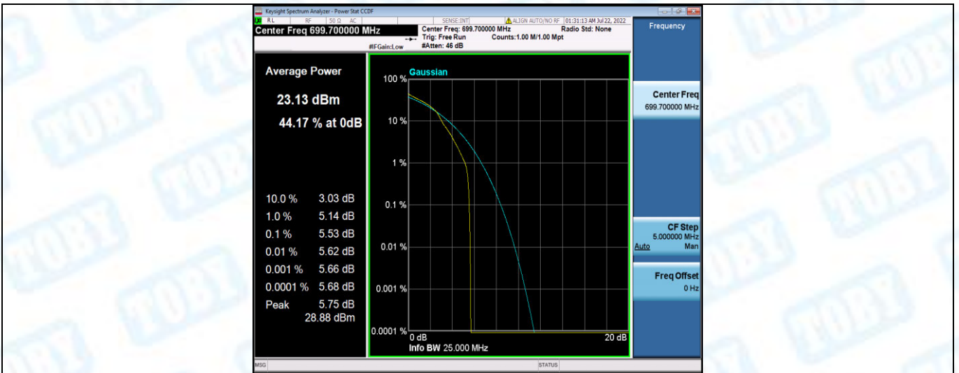
Band12-1.4MHz-16QAM-23017-6RB#0
