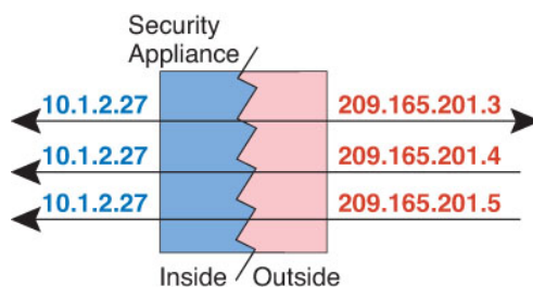
Figure 56: One-to-Many Static NAT
