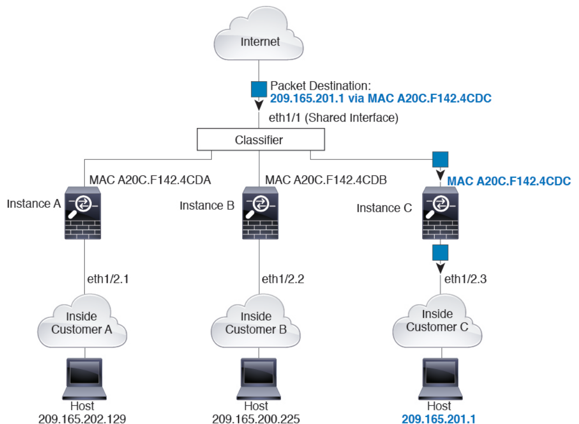
Figure 18: Packet Classification with a Shared Interface Using MAC Addresses
