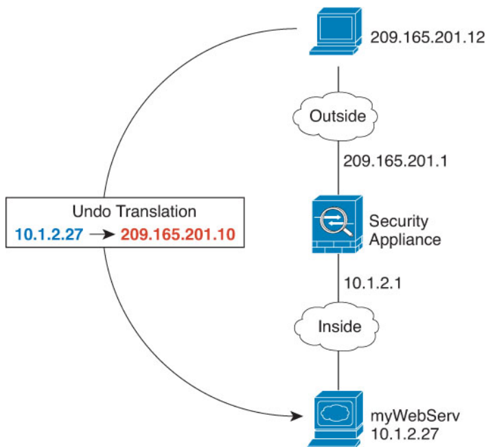
Figure 61: Static NAT for an Inside Web Server
