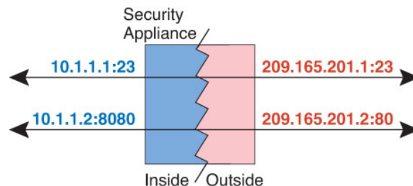
Figure 55: Typical Static NAT with Port Translation Scenario
