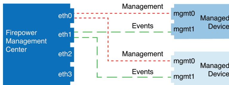
Figure 46: Separate Event Interface on the Firepower Management Center and Managed Devices
