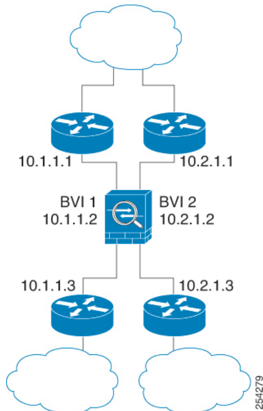
Figure 10: Transparent Firewall Network with Two Bridge Groups
