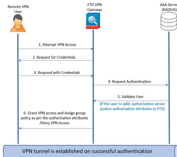
Figure 39: Remote Access VPN Group Policy Selection by AAA Server
