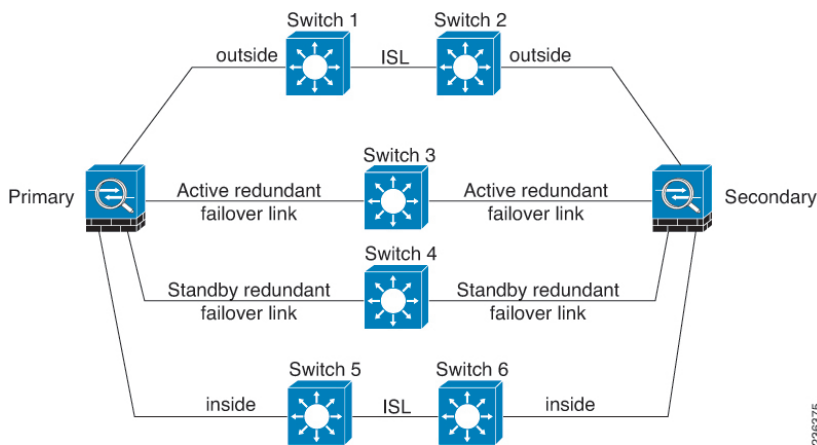
Figure 31: Connecting with Inter-switch Links
