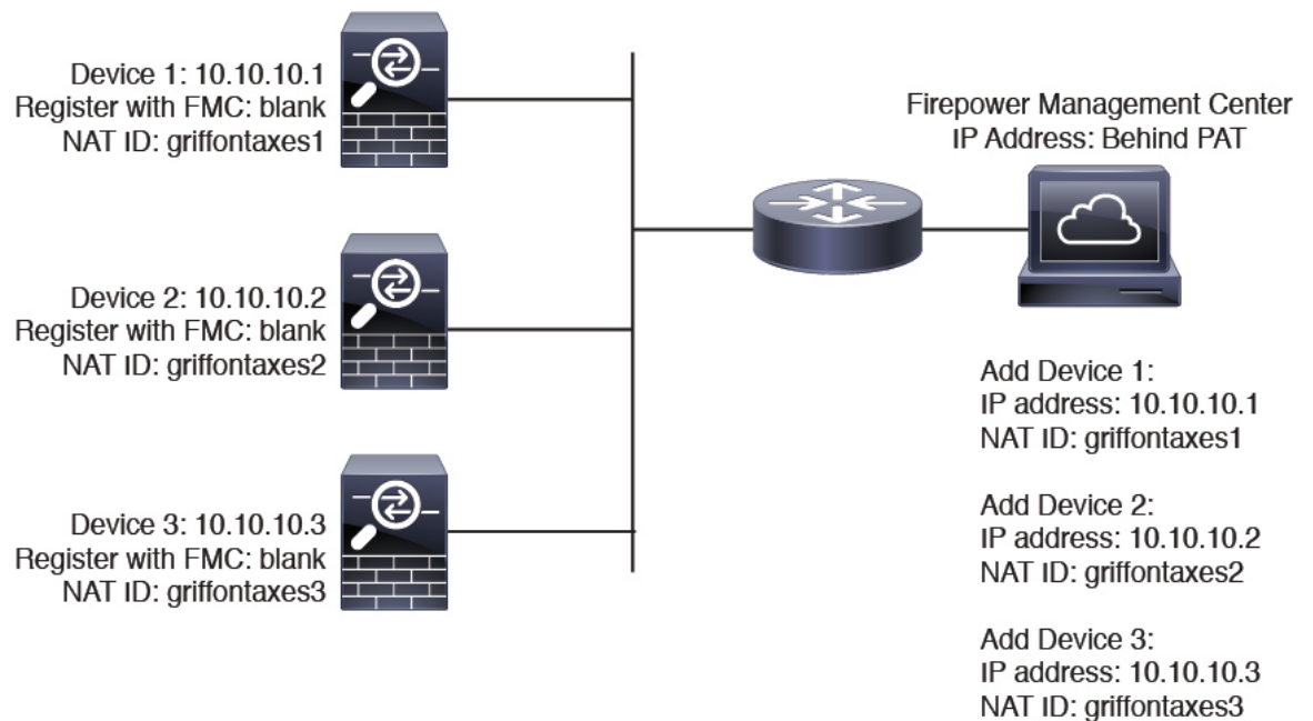
Figure 43: NAT ID for FMC Behind PAT
