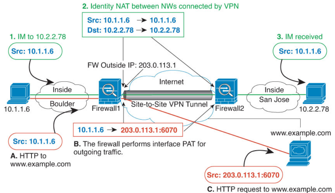
Figure 67: Interface PAT and Identity NAT for Site-to-Site VPN
