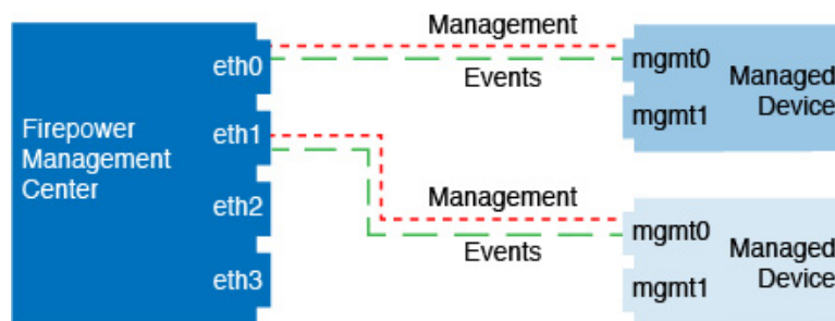
Figure 45: Multiple Management Interfaces on the Firepower Management Center
