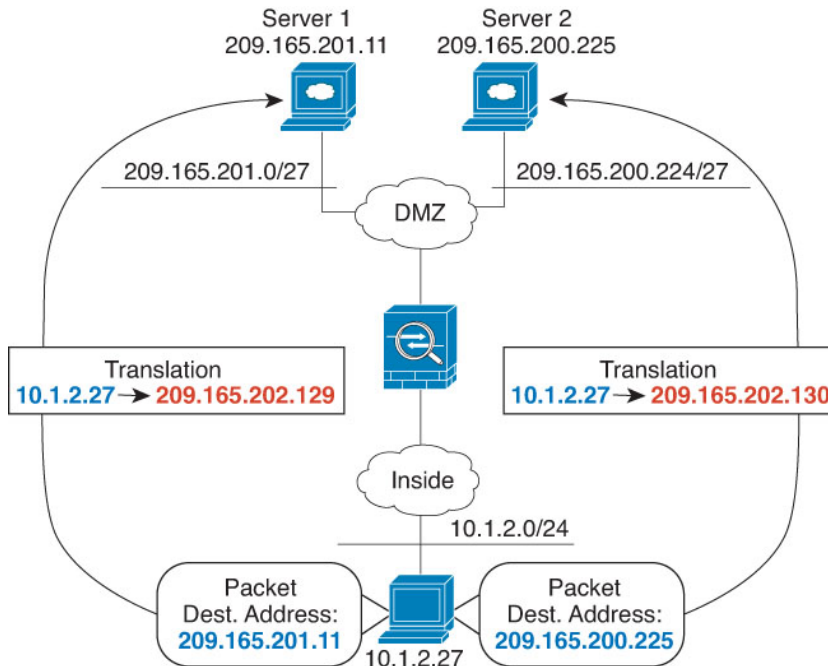
Figure 65: Manual NAT with Different Destination Addresses
