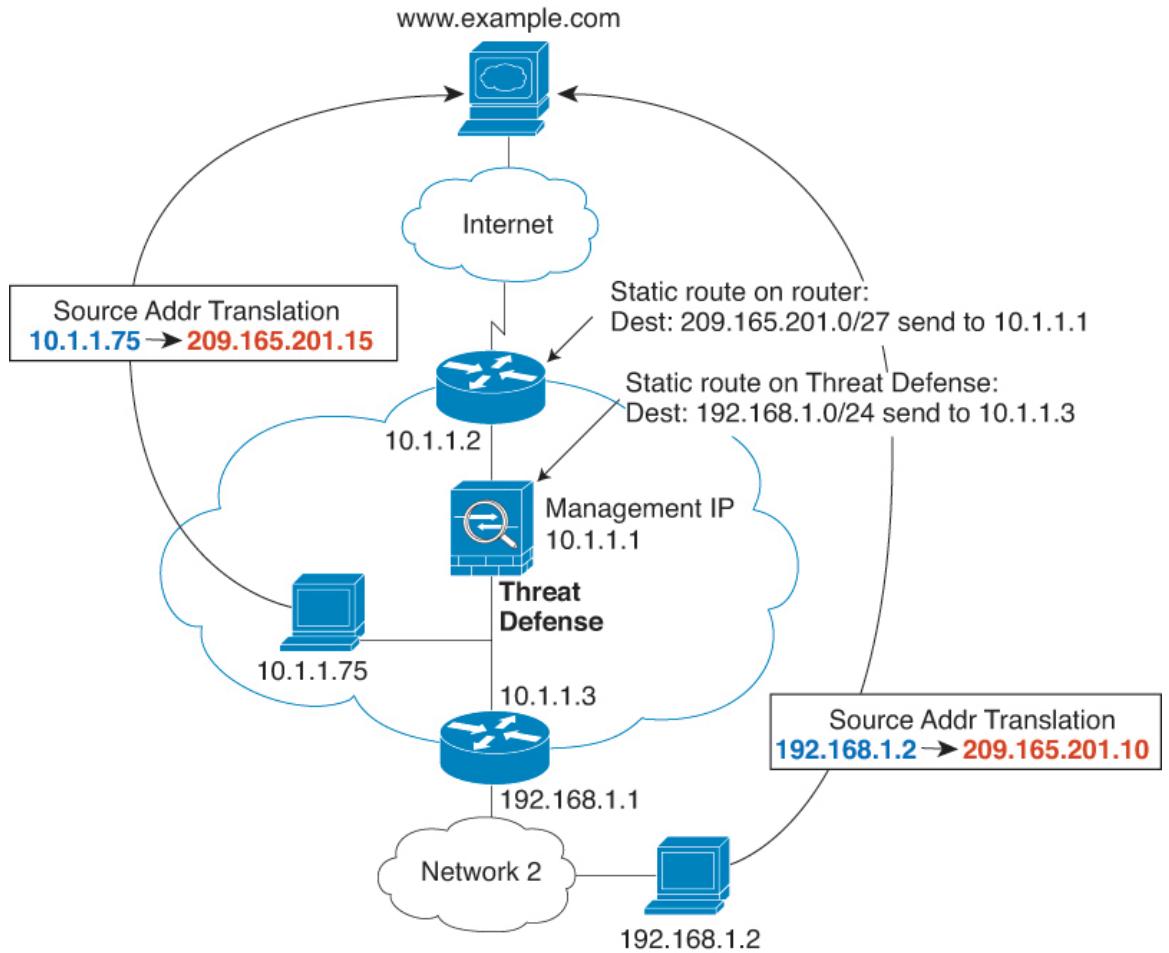
Figure 12: NAT Example: NAT within a Bridge Group
