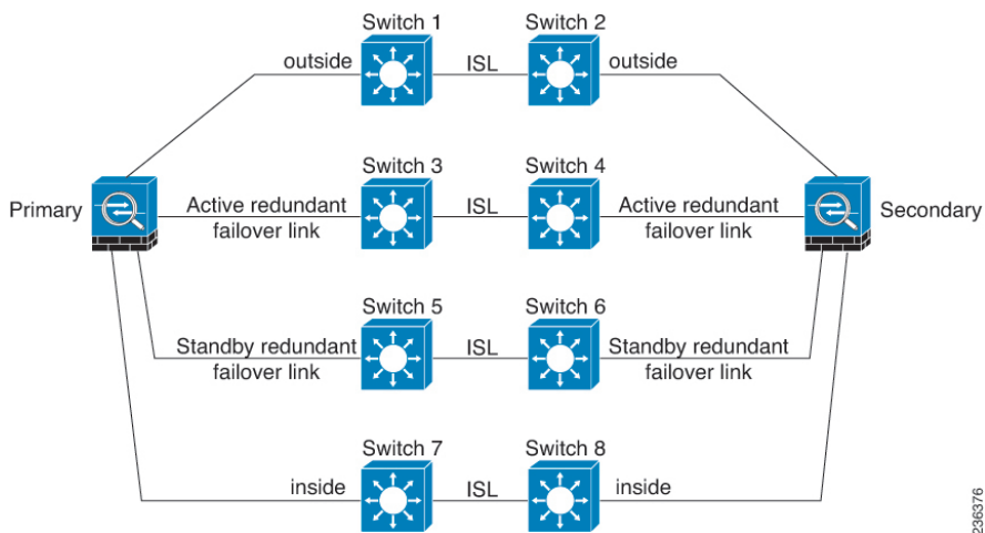
Figure 31: Connecting with Inter-switch Links
