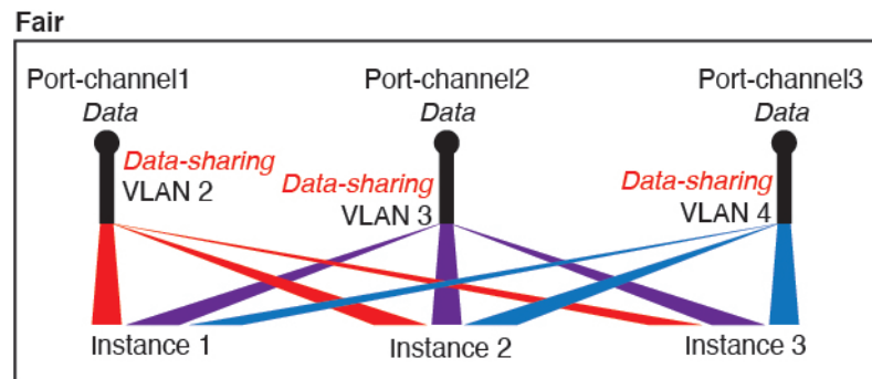
Figure 16: Fair: Shared Subinterfaces on Separate Parents
