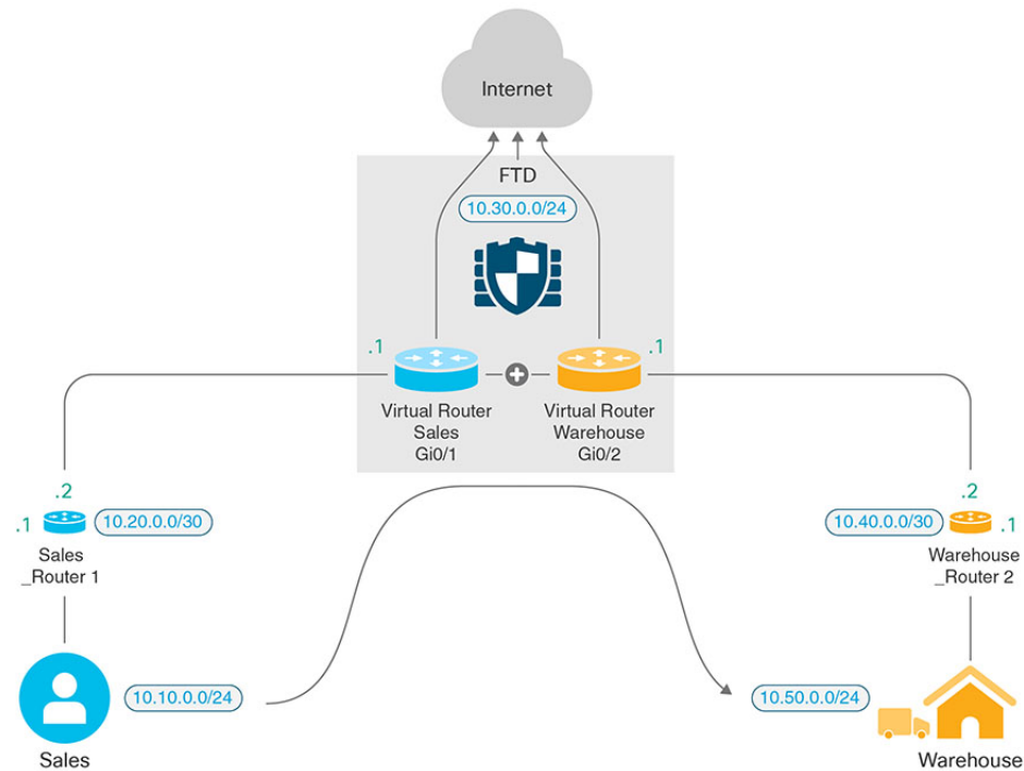
Figure 38: Interconnecting Two Virtual Routers - An Example
