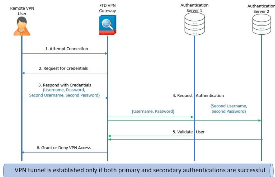
Figure 40: Remote Access VPN Secondary or Double Authentication
