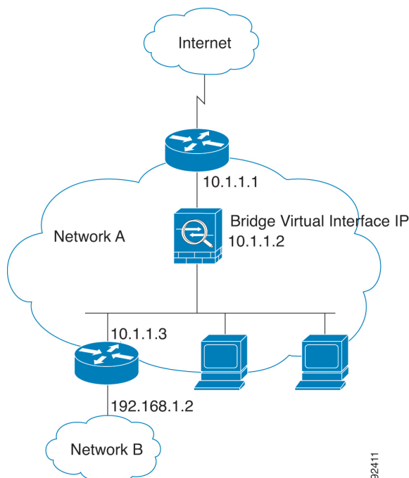
Figure 9: Transparent Firewall Network
