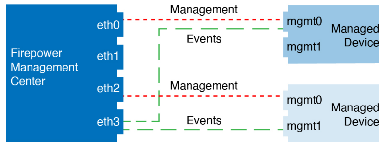
Figure 47: Mixed Management and Event Interface Usage
