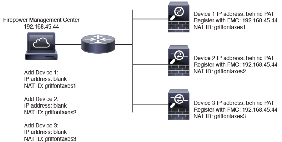
Figure 42: NAT ID for Managed Devices Behind PAT
