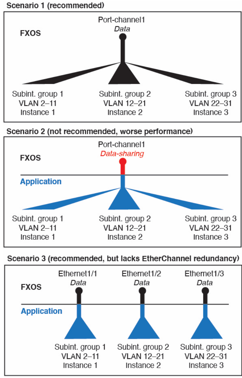
Figure 13: VLANs in FXOS vs. the Application for Container Instances
