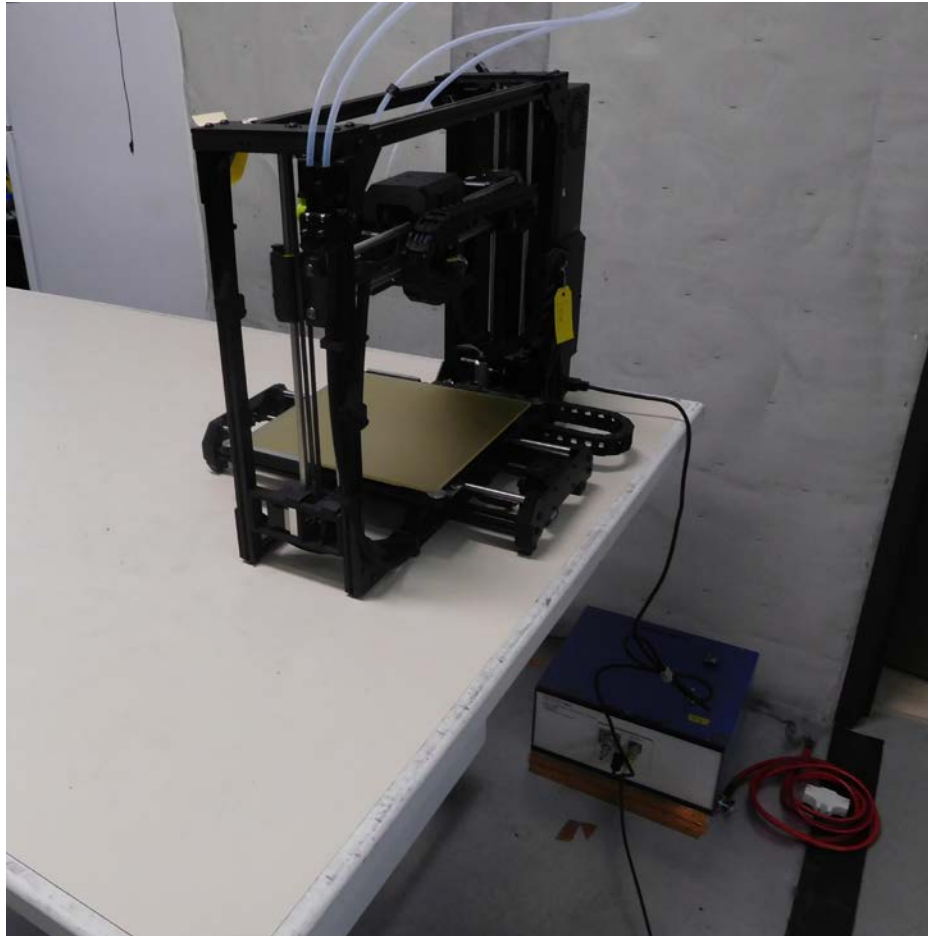
Conducted emissions test setup
