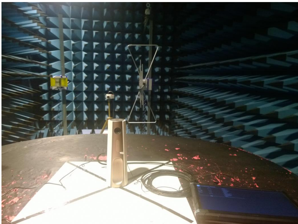
Radiated Emission 18GHz-26.5GHz
