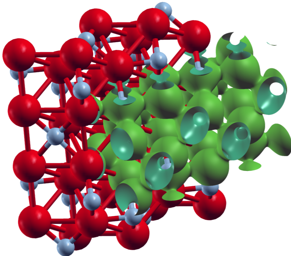
Figure 4.5: XCrySDen plot of an isosurface for the total charge density for \text{Fe}_2\text{N} .
