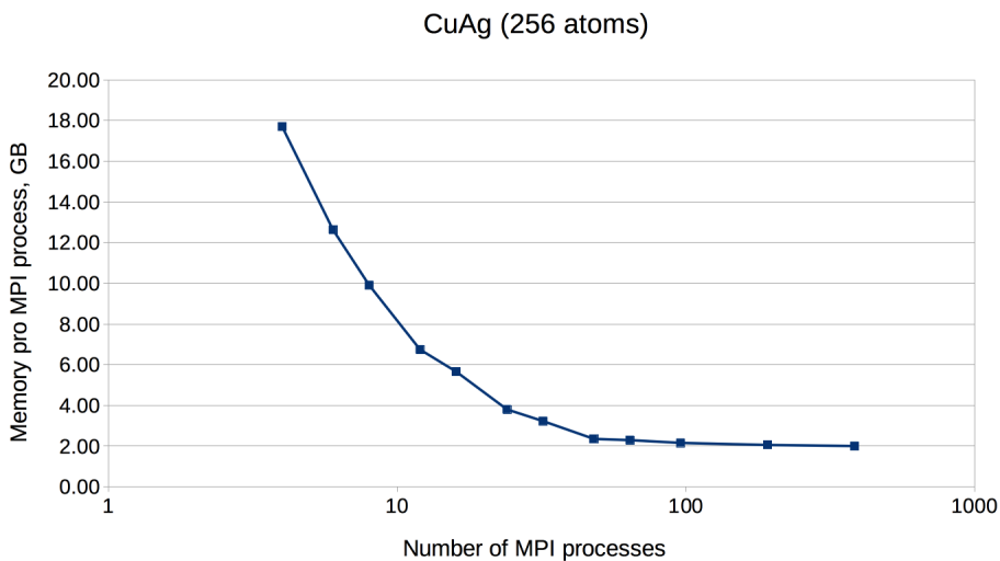
Figure 5.3: An example of FLEUR memory requirements depending on the amount of MPI ranks. Test system: CuAg (256 atoms, 1 k point). Memory usage was measured on the CLAIX supercomputer (Intel E5-2650V4, 2.2 GHz, 128 GB per node).
