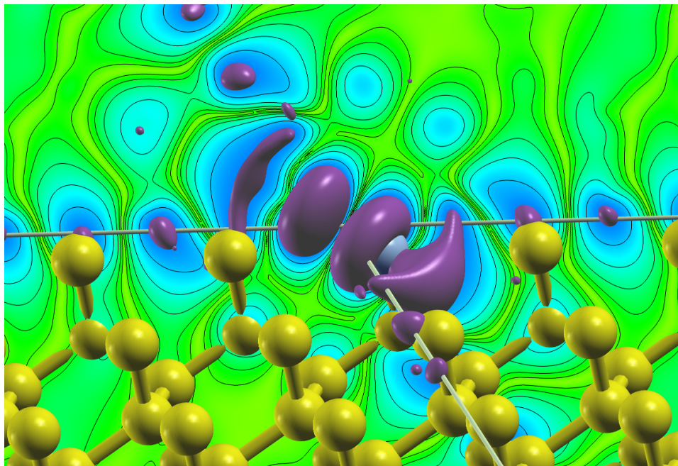
Figure 4.7: Density due to defect states of an A-nitrogen center defect in diamond.
