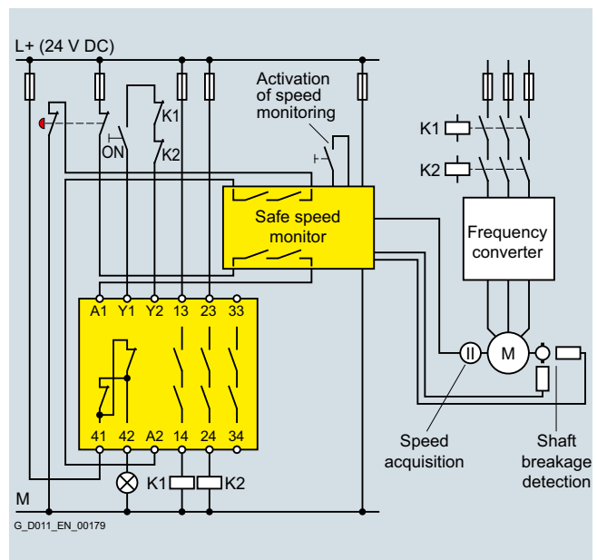
Conventional wiring
