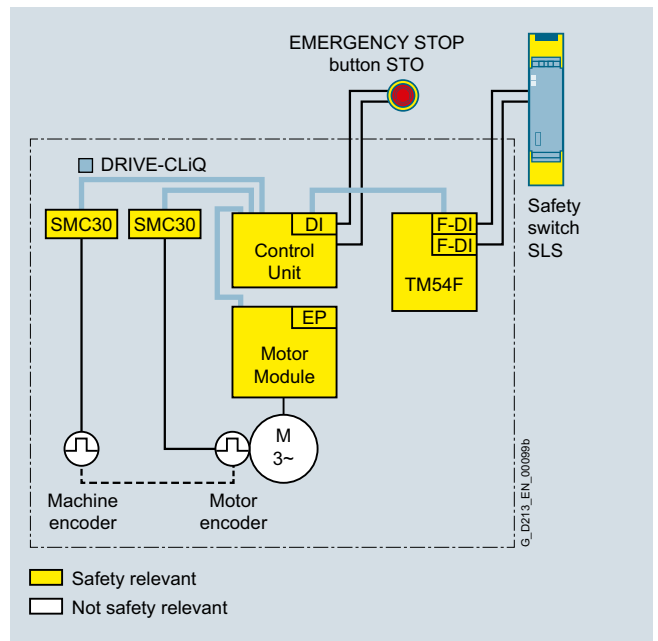
Integrated safety via fail-safe inputs
