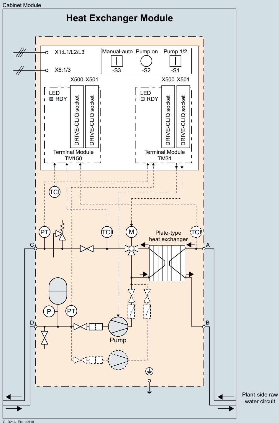
Connection example: Heat Exchanger Module, liquid-cooled
