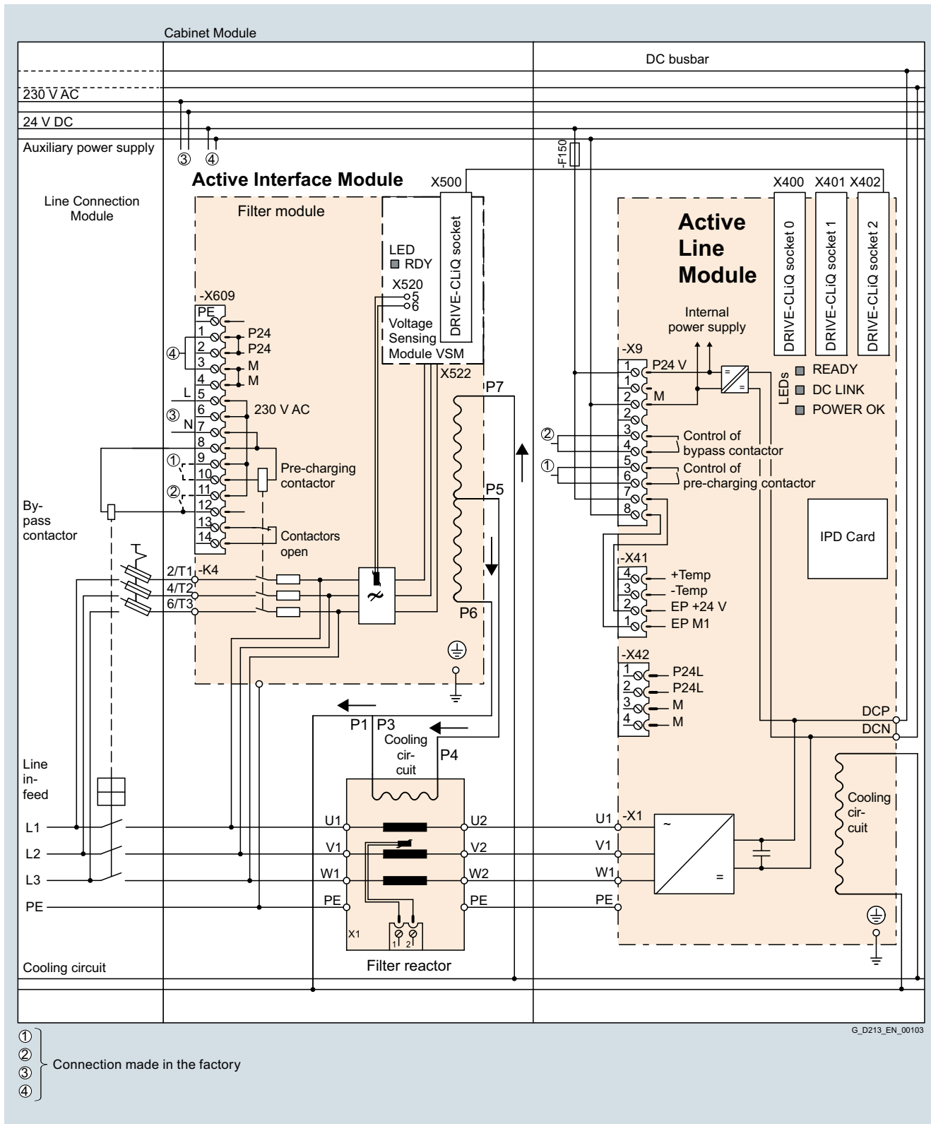
Connection example: Active Line Connection Module, liquid-cooled
