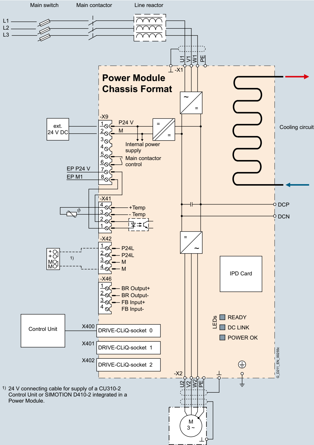
Connection example of a liquid-cooled Power Module in the chassis format
