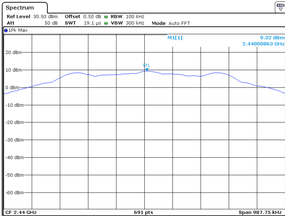
Channel 19 (2440MHz) Reference Level: 9.32dBm
