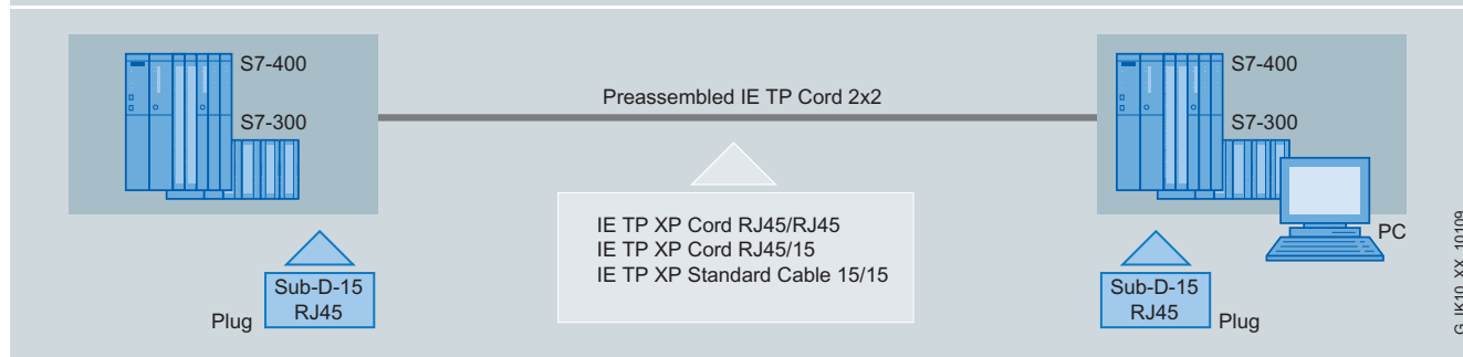
IE TP Cord can be used to directly connect individual components (10/100 Mbit/s)
