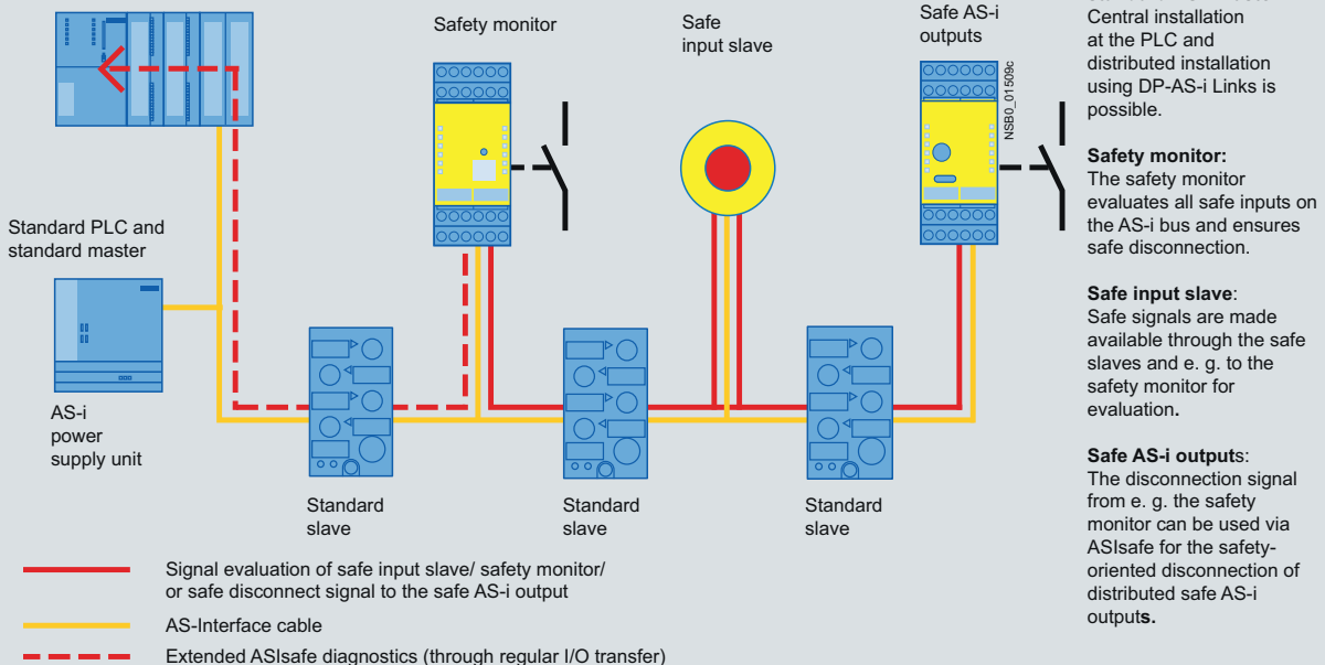
The ASIsafe components and their signal flows
