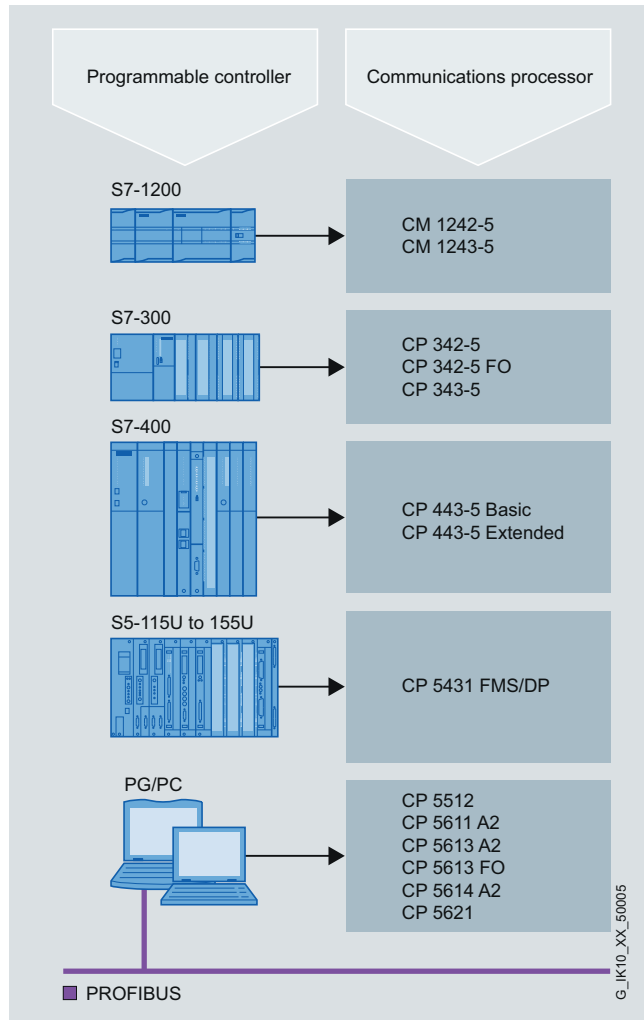
PROFIBUS system connections for SIMATIC and PC
