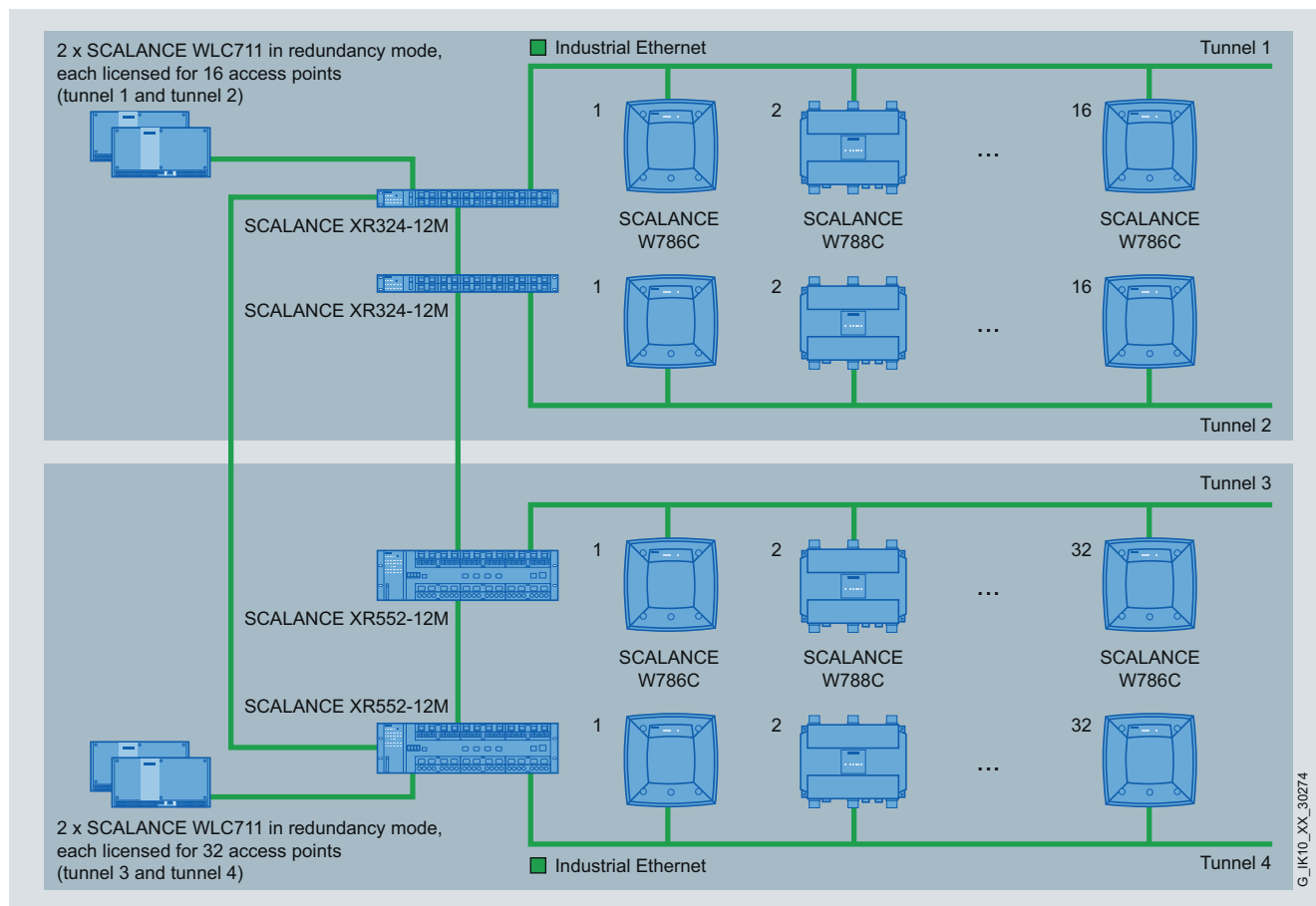
SCALANCE WLC711 IWLAN Controller in redundancy mode
