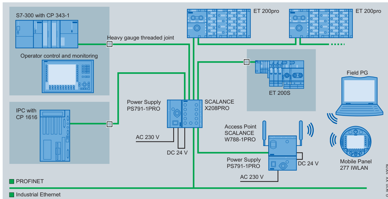
Example for the use of power supply PS791-1PRO with SCALANCE X and SCALANCE W
