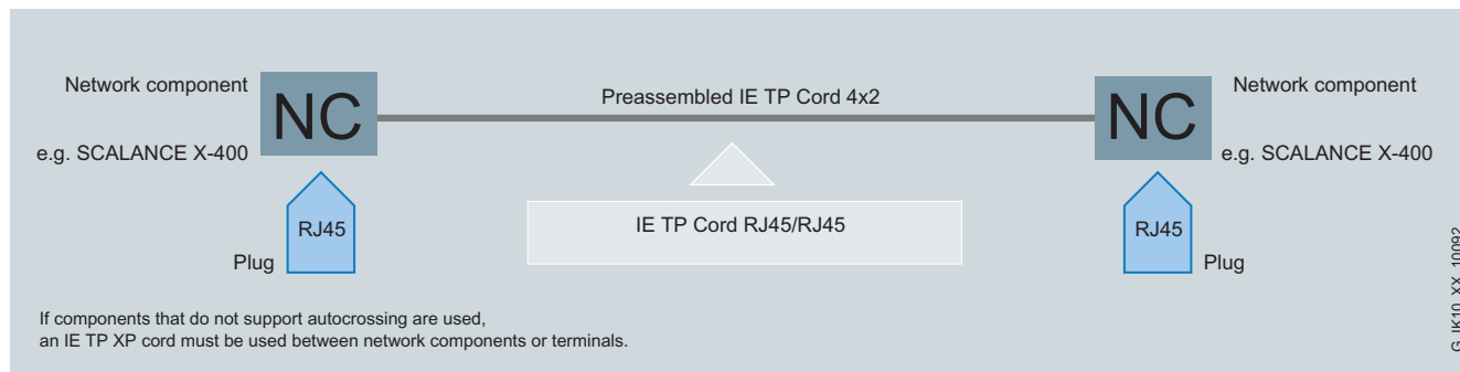
IE TP Cord RJ45/RJ45 can be used to directly connect individual components (10/100/1000 Mbit/s)
