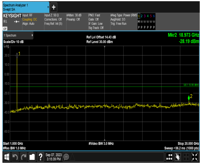
Band4-1.4MHz-16QAM-20175-1RB#0-Range1:30~1000MHz
