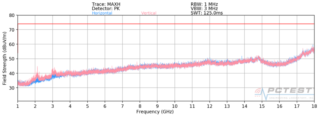
Plot 7-2. Radiated Spurious Plot above 1GHz (Configuration 1)
