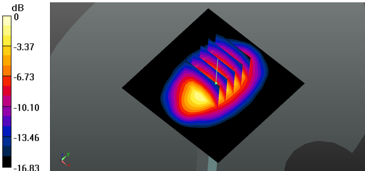
0 dB = 12.8 W/kg
