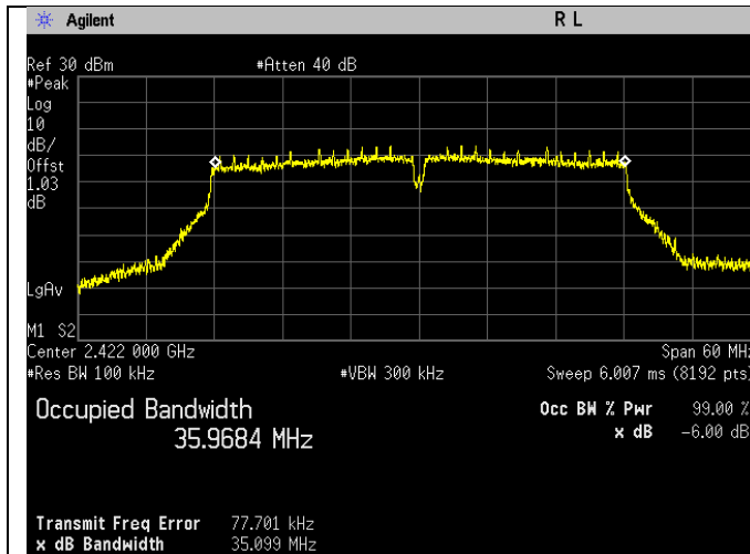
6dB Bandwidth. 802.11n Frequency 2422 MHz
