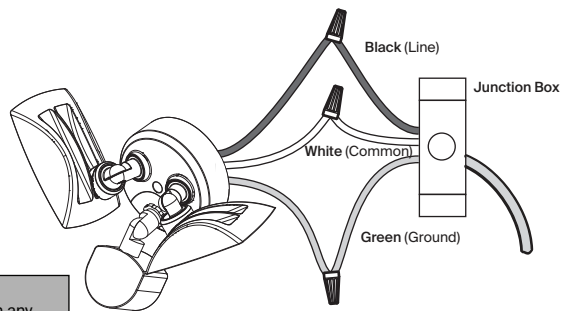
Non-Dimming Wiring Diagram
