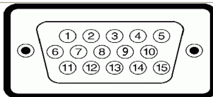
VGA Connector layout
