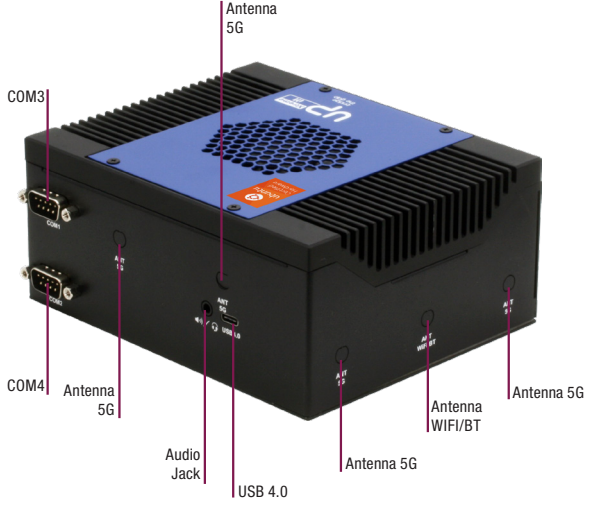
Rear View
