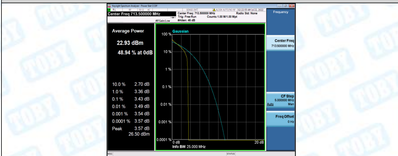
Band12-5MHz-QPSK-23155-25RB#0
