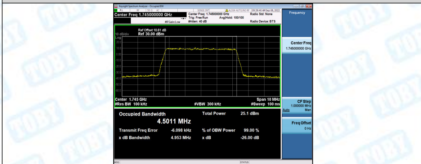
Band66-5MHz-16QAM-132647-25RB#0
