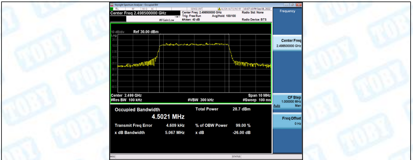
Band41-5MHz-QPSK-40620-25RB#0
