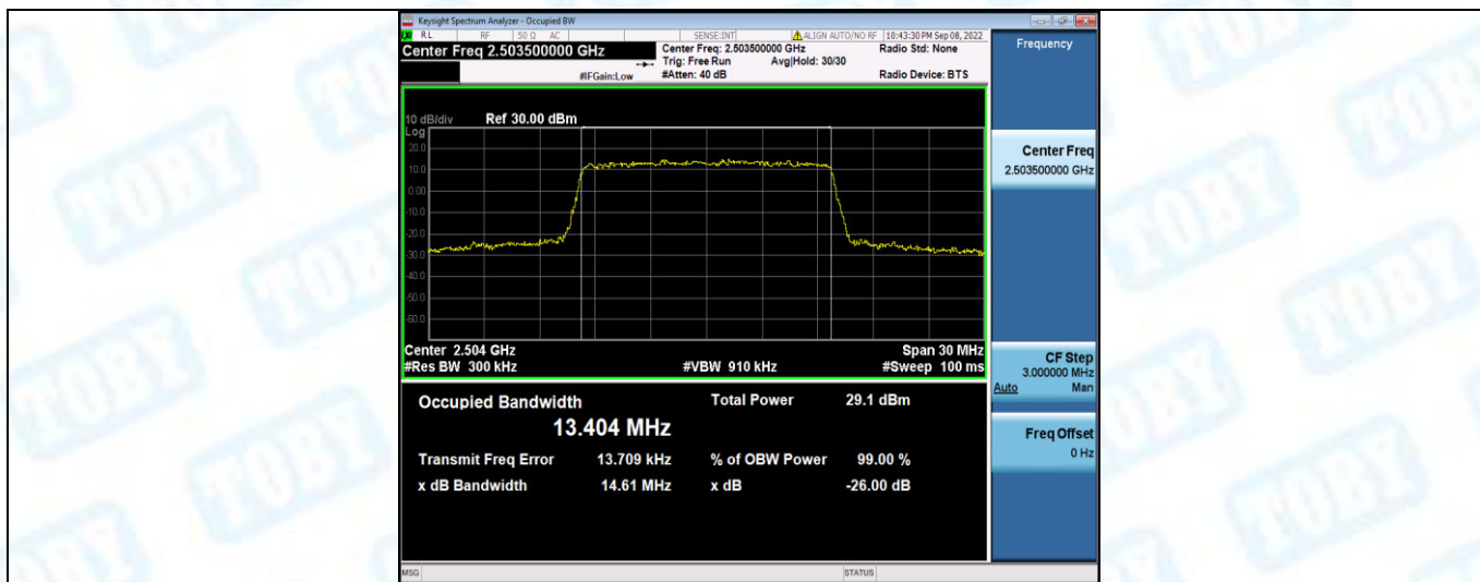
Band41-15MHz-QPSK-40620-75RB#0
