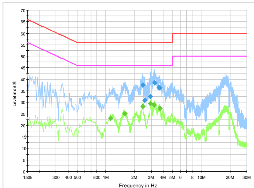
Fig.35. AC Powerline Conducted Emission-ch19
