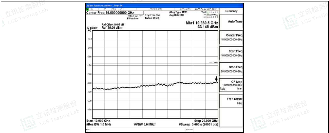
Band4-20MHz-16QAM-20050-1RB#0-Range1:0.009~0.15MHz
