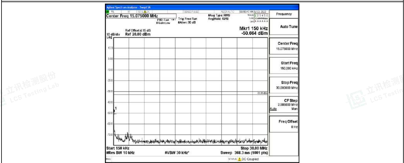
Band4-20MHz-QPSK-20175-1RB#0-Range3:30~100MHz
