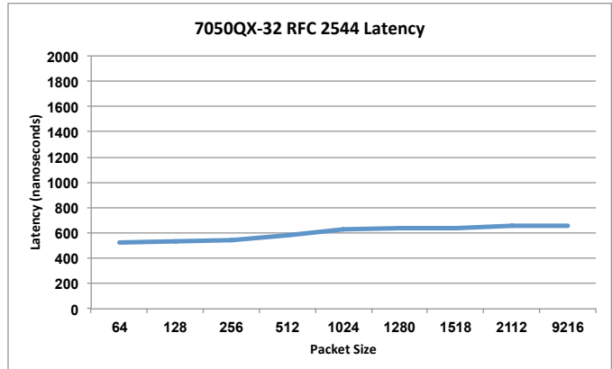
Arista 7050QX: Latency through QSFP+ ports
