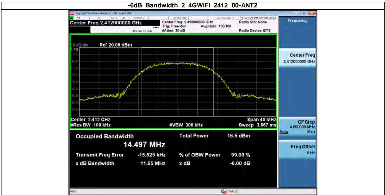
-6dB_Bandwidth_2_4WiFi_2437_00-ANT2
