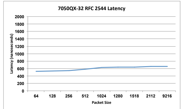
Arista 7050QX: Latency through QSFP+ ports
