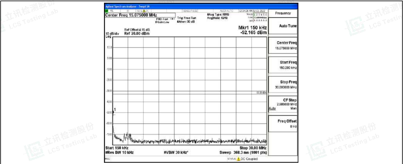
Band2-5MHz-QPSK-19175-1RB#0-Range3:30~1000MHz
