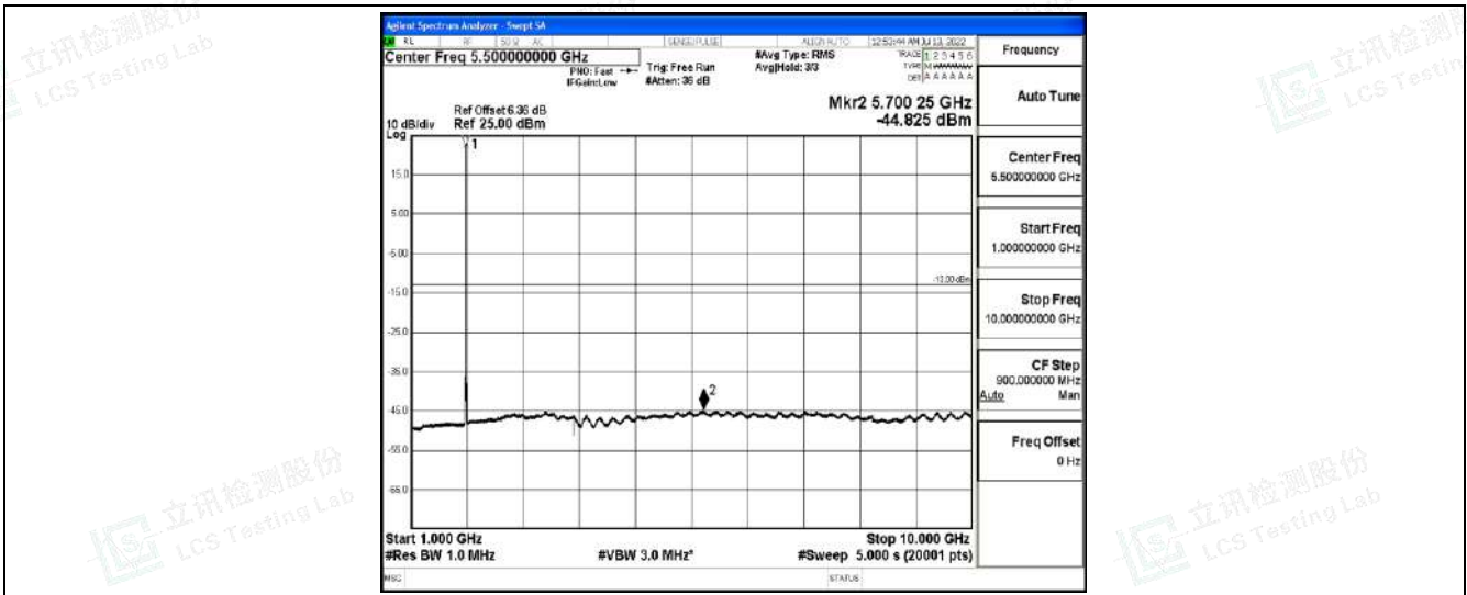
Band2-10MHz-QPSK-18900-1RB#0-Range5:10000~20000MHz
