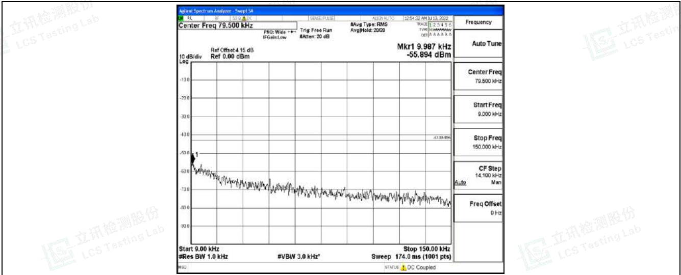
Band2-10MHz-16QAM-18900-1RB#0-Range2:0.15~30MHz
