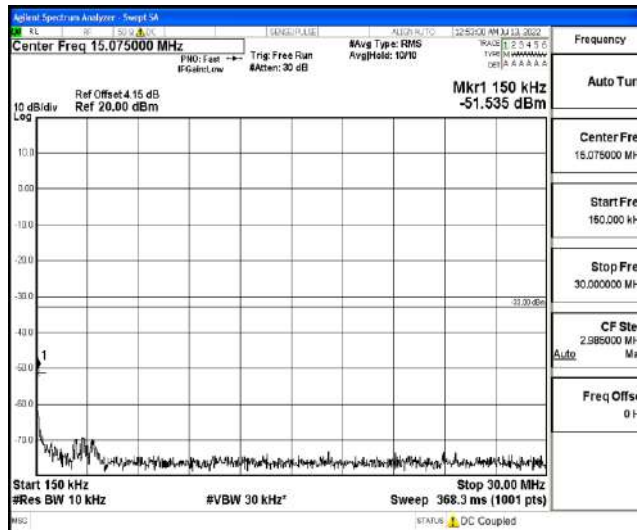
Band2-10MHz-QPSK-18900-1RB#0-Range3:30~100MHz
