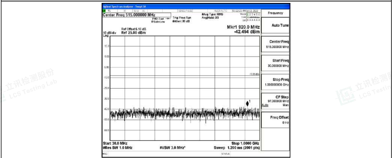
Band2-15MHz-QPSK-19125-1RB#0-Range4:1000~10000MHz
