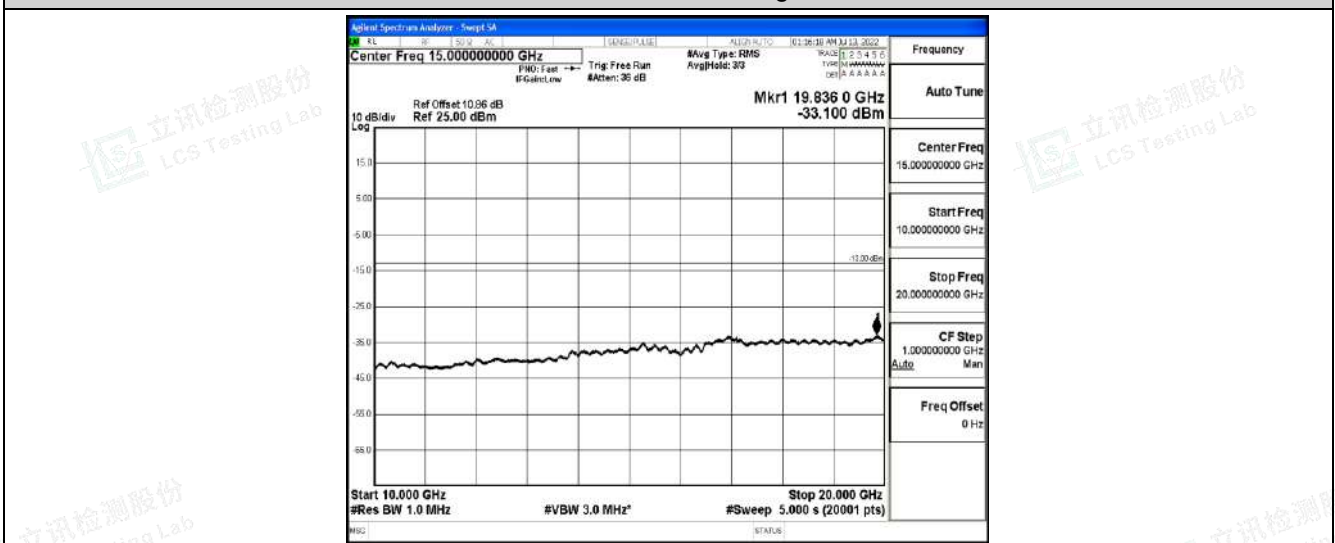
Band2-15MHz-QPSK-18900-1RB#0-Range1:0.009~0.15MHz
