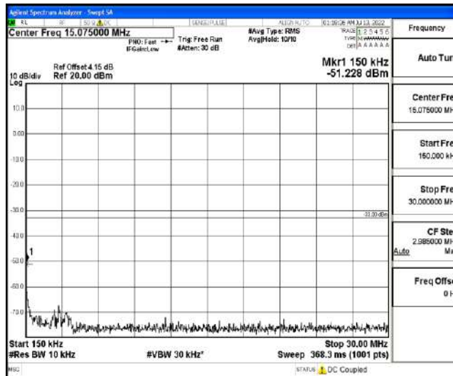
Band2-15MHz-QPSK-18900-1RB#0-Range3:30~100MHz
