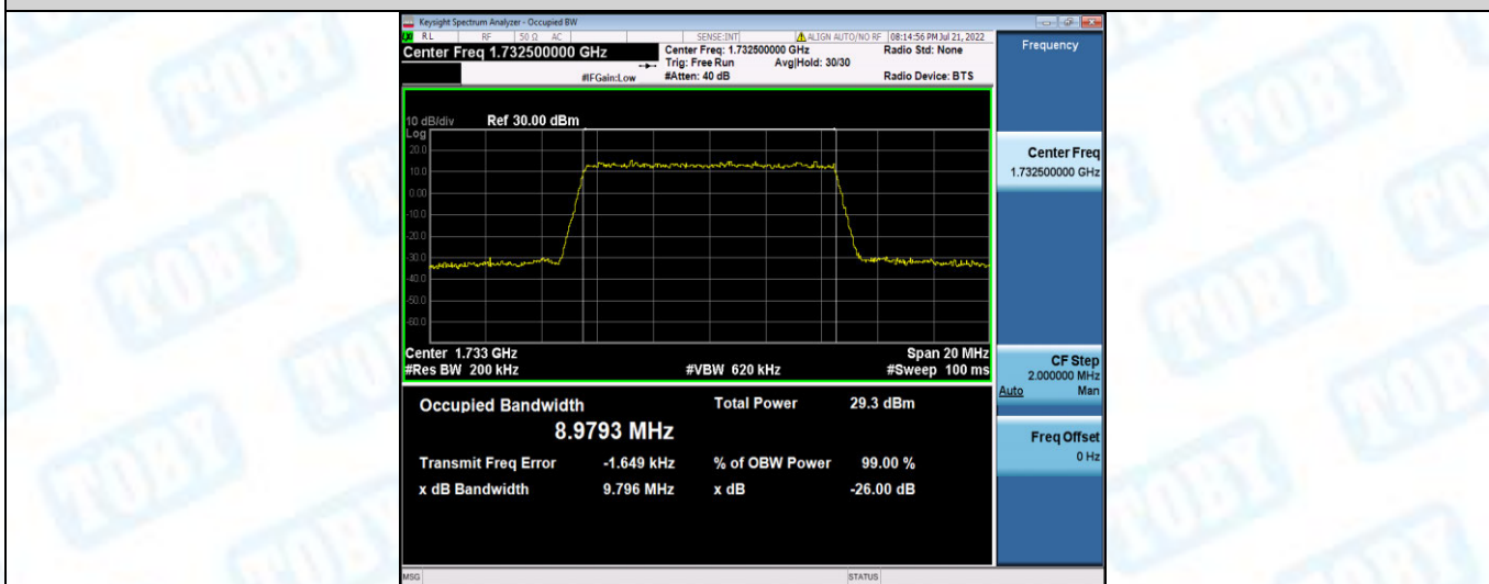
Band4-10MHz-16QAM-20350-50RB#0
