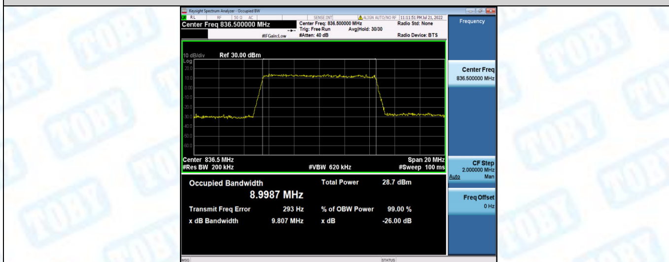
Band5-10MHz-16QAM-20600-50RB#0
