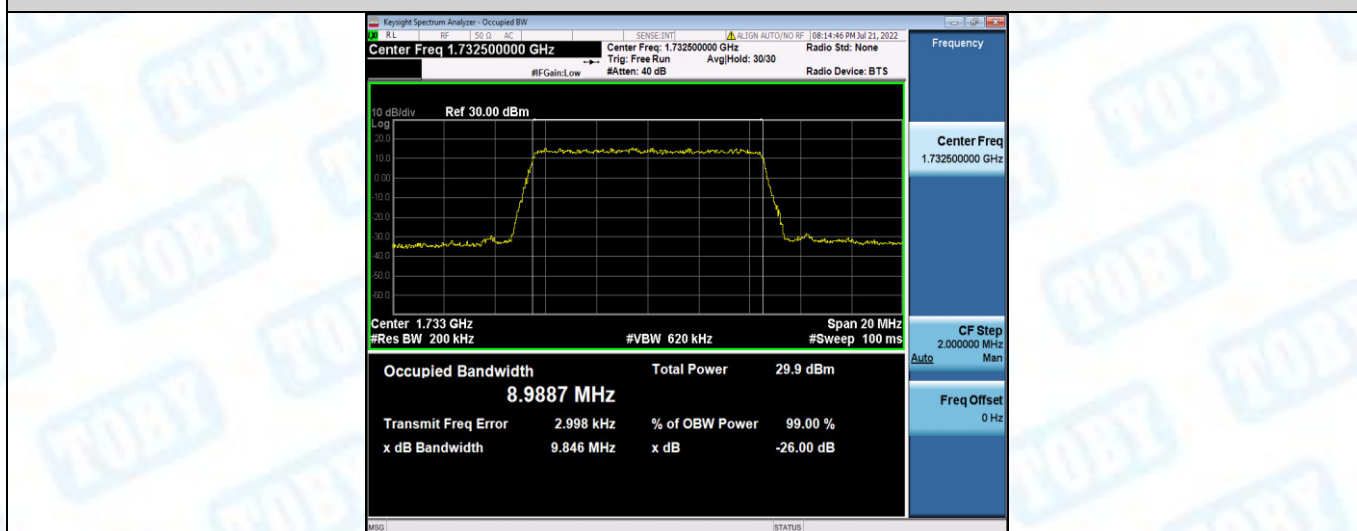
Band4-10MHz-QPSK-20350-50RB#0
