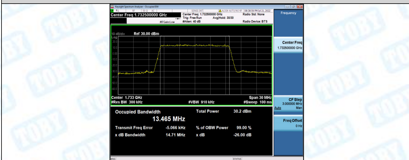
Band4-15MHz-QPSK-20325-75RB#0
