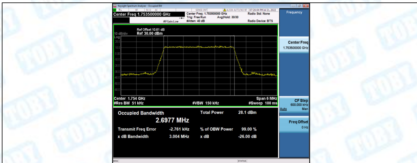
Band4-5MHz-QPSK-19975-25RB#0
