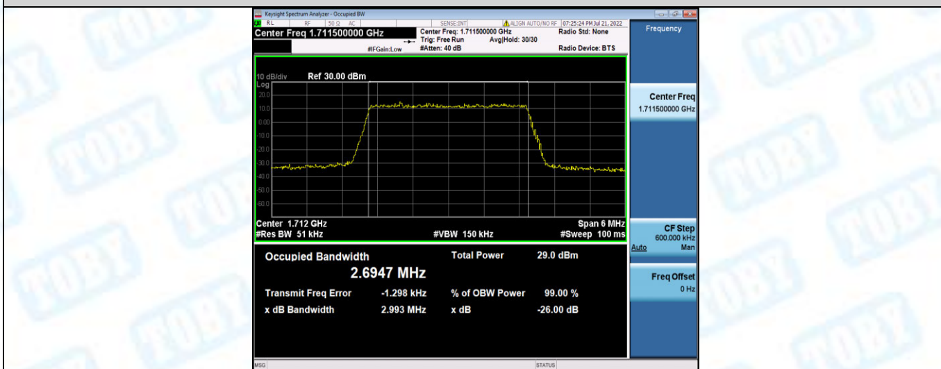
Band4-3MHz-16QAM-20175-15RB#0
