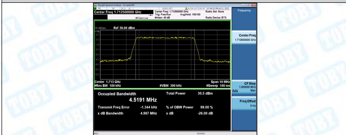
Band4-5MHz-QPSK-20175-25RB#0
