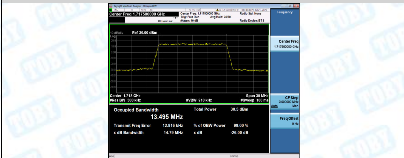
Band4-15MHz-QPSK-20175-75RB#0
