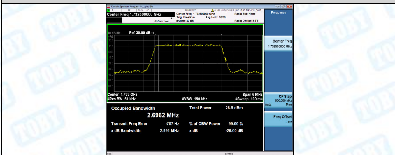
Band4-3MHz-16QAM-20385-15RB#0
