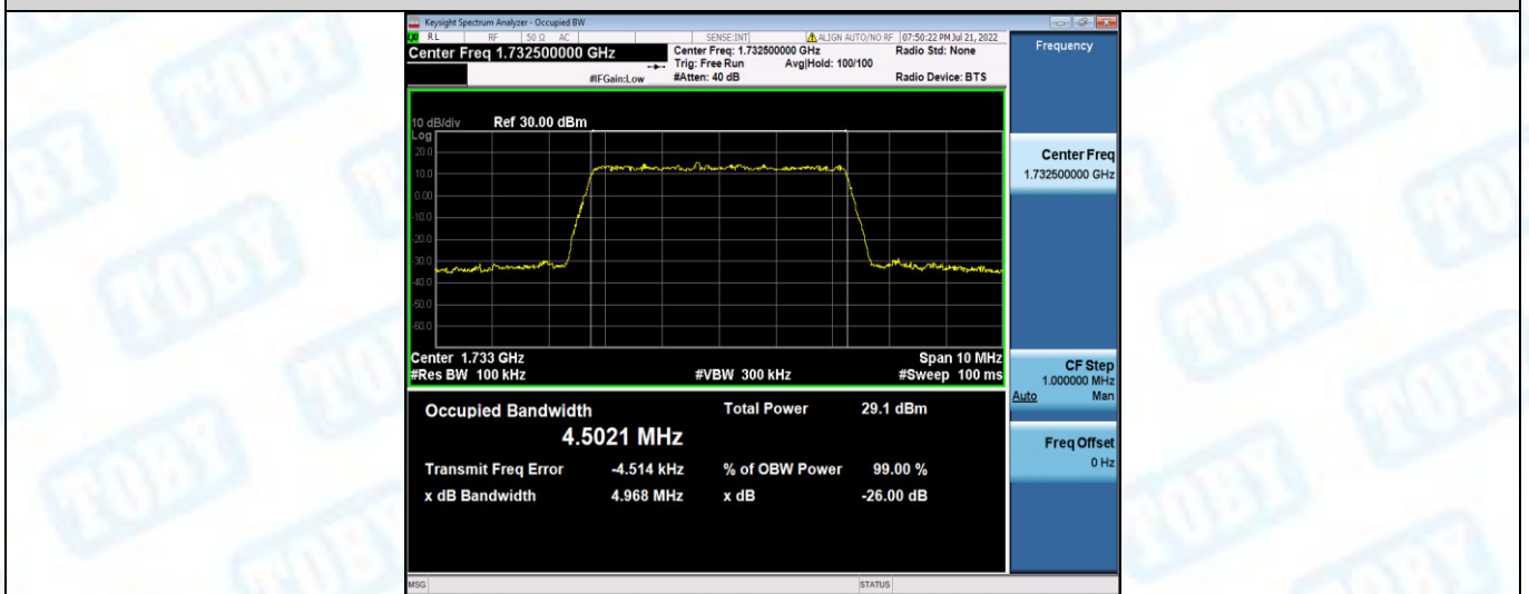
Band4-5MHz-16QAM-20375-25RB#0
