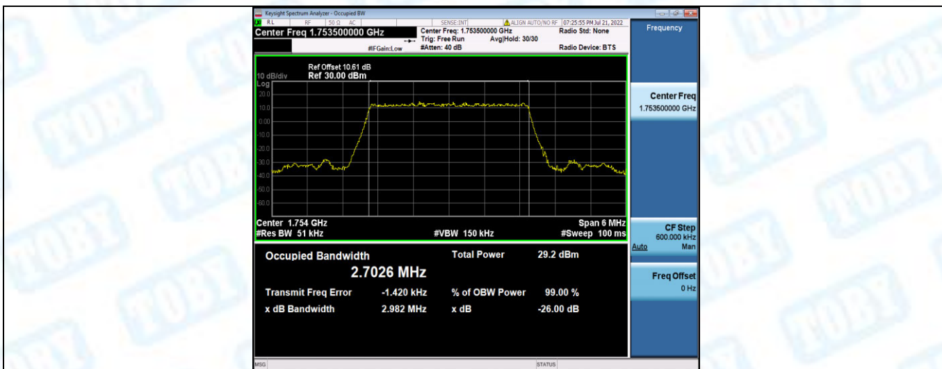
Band4-3MHz-16QAM-19965-15RB#0
