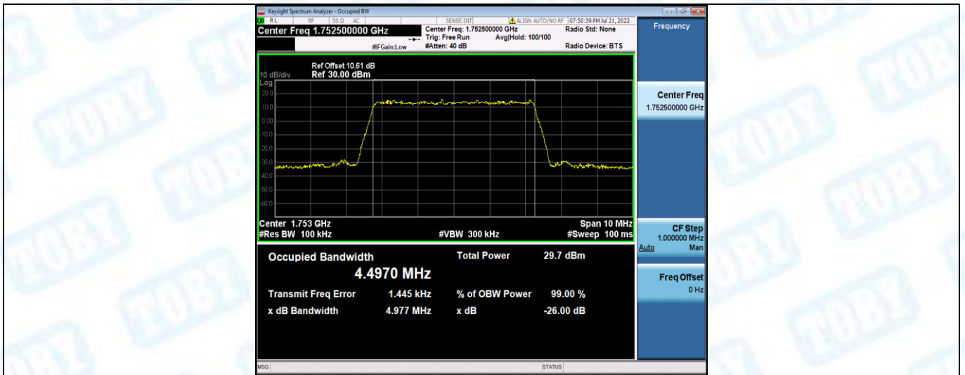
Band4-5MHz-16QAM-19975-25RB#0
