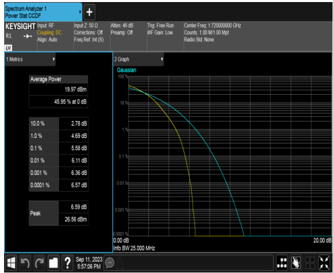
Band66-20MHz-16QAM-132322-1RB#0
