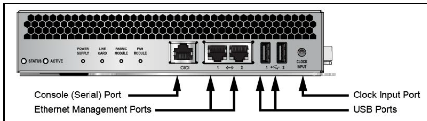
Figure 17: Supervisor Ports
