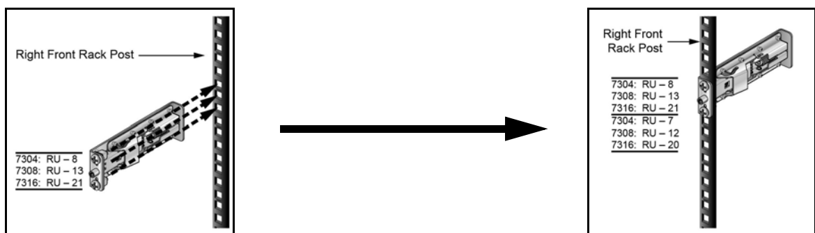
Figure 11: Attaching the Right Mounting Ear
