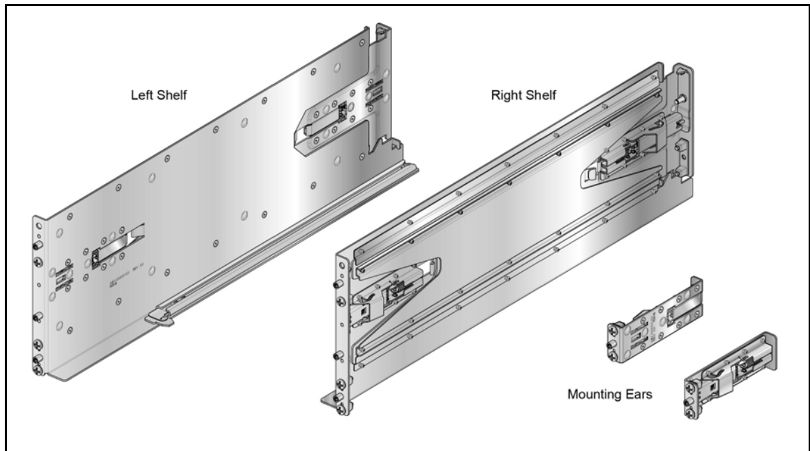
Figure 26: Four-Post Rack Mount Parts
