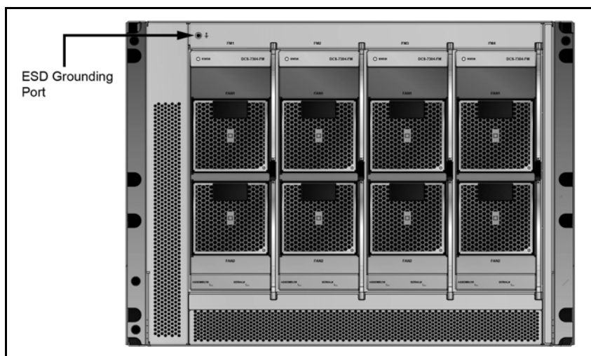
Figure 15: ESD Grounding Port – Rear Panel
