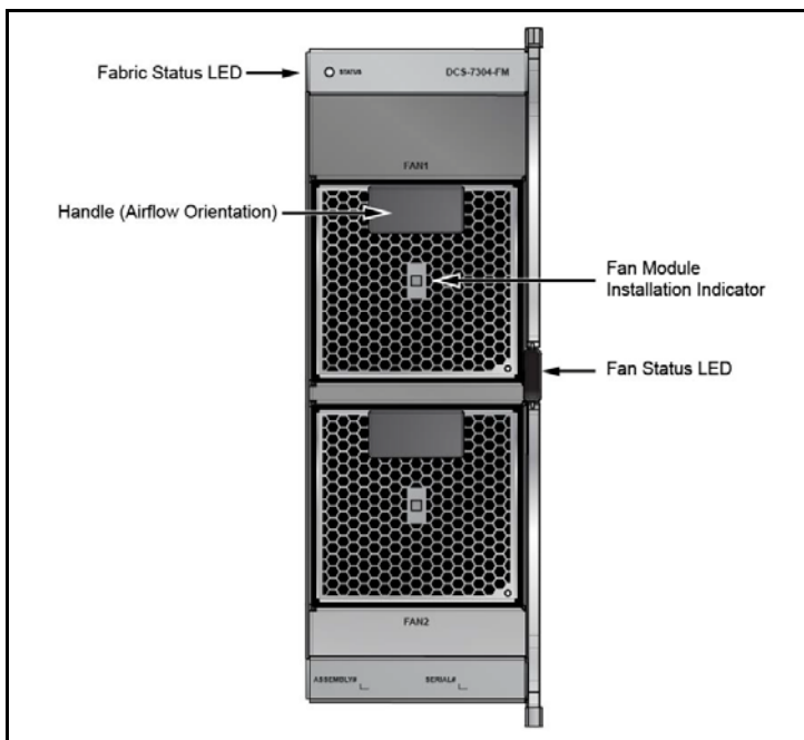
Figure 21: Fan Status and Fabric Status LEDs
