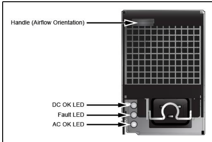
Figure 22: Power Supply
