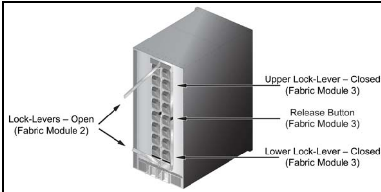
Figure 23: Fabric Module Locking Mechanisms
