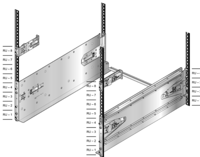
Figure 7: Component Placement
