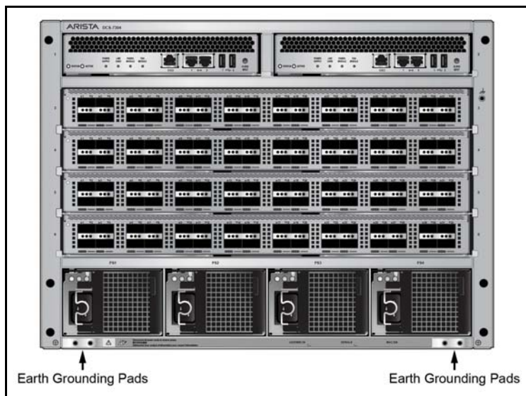
Figure 14: Grounding Pad and ESD Grounding Port Sockets
