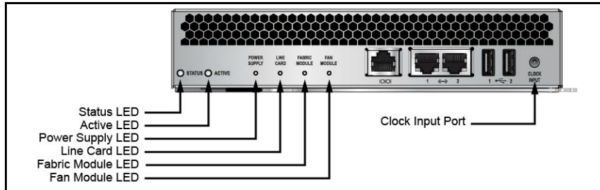
Figure 19: Supervisor Module
