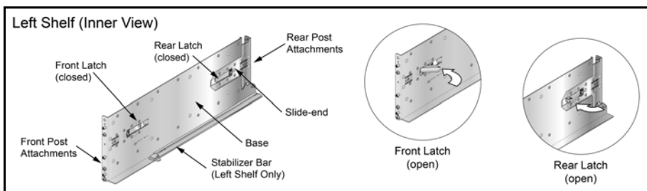
Figure 4: Left Shelf – Inner View
