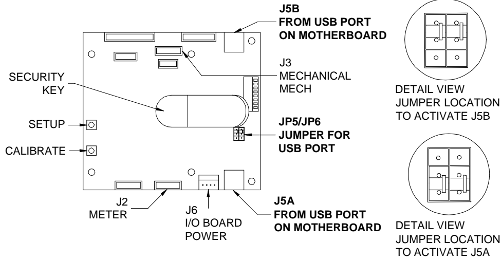
FIGURE 27 - I/O BOARD DRAWING
