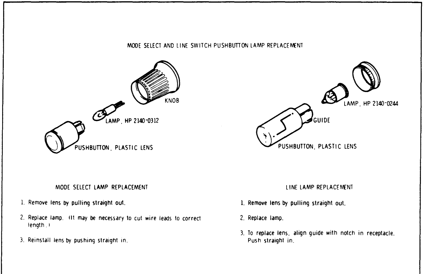
Figure 3-3. Lamp Replacement
