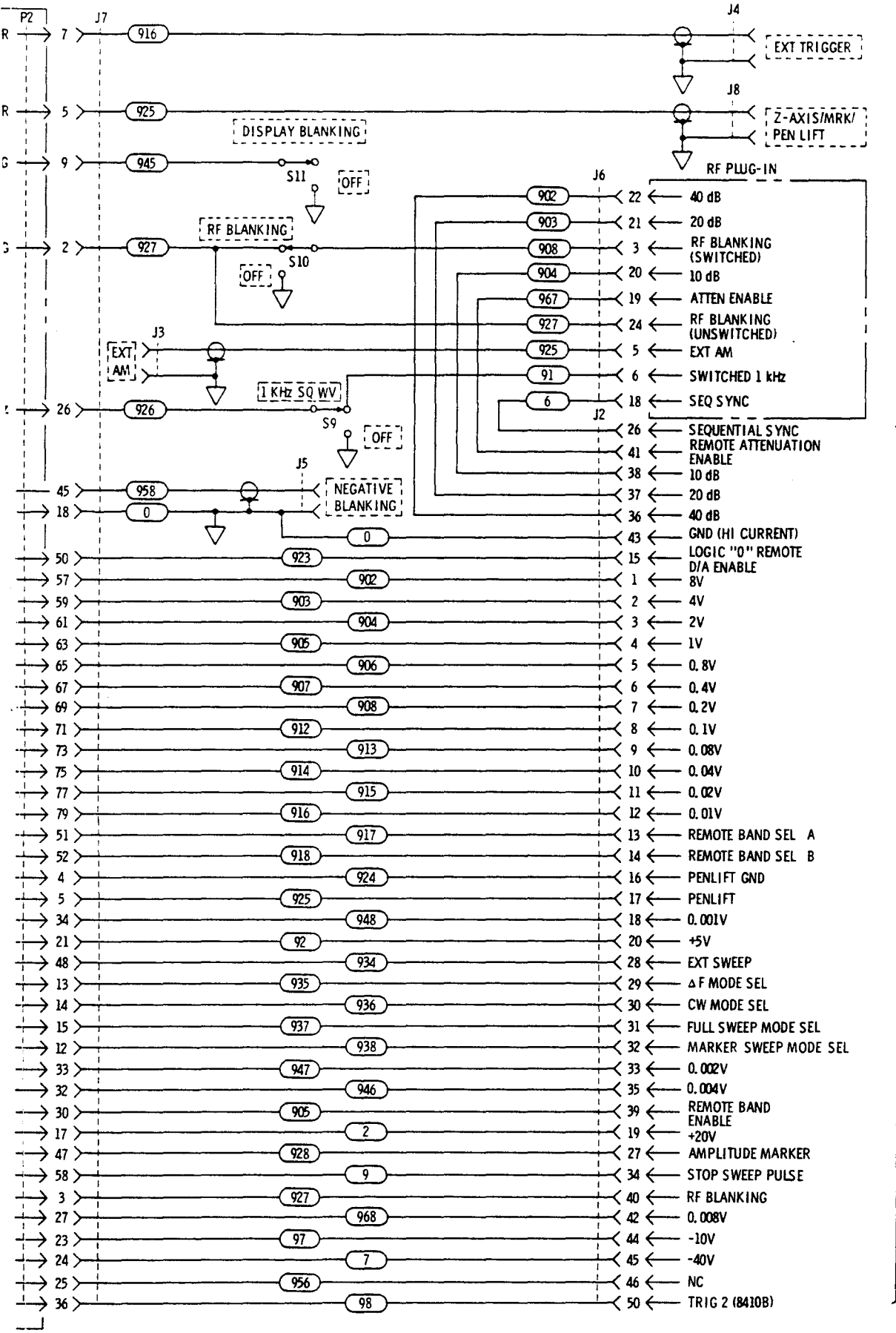
Figure 8-37. Rear Panel Wiring Diagram
