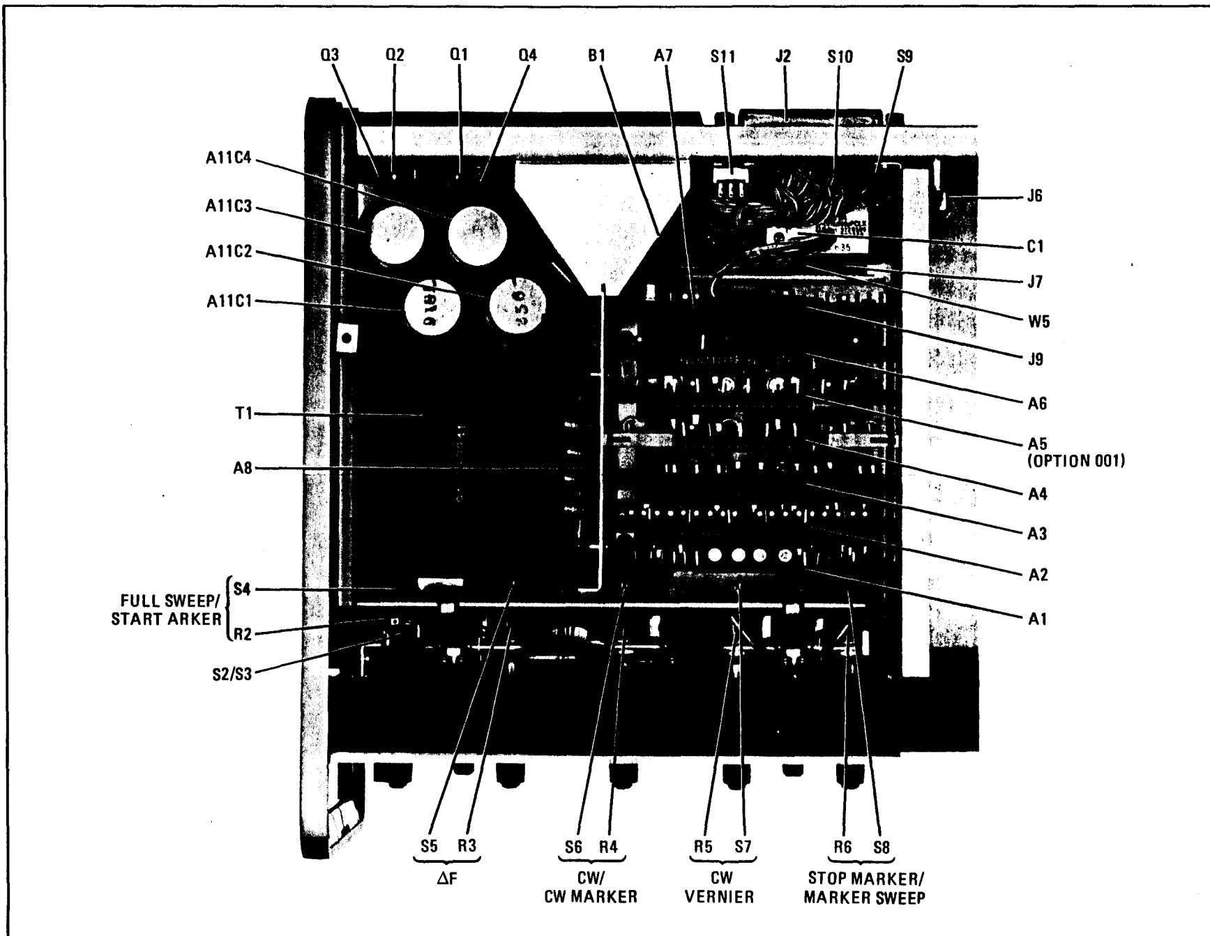
Figure 8-38. Top View, Major Assembly and Component Locations
