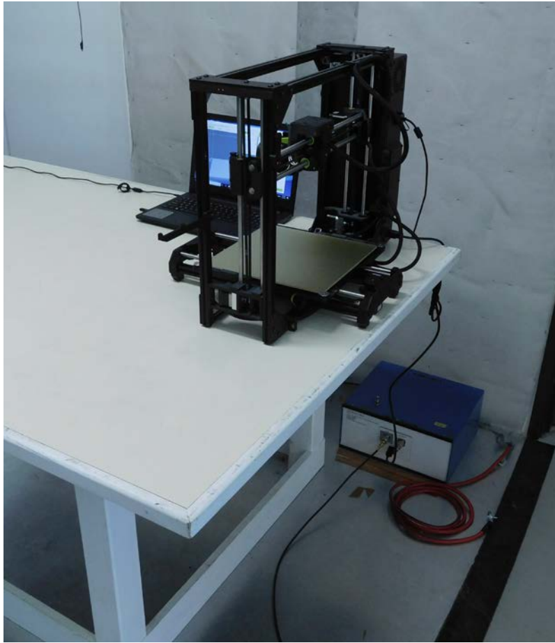
Conducted emissions test setup – connected through usb cable
