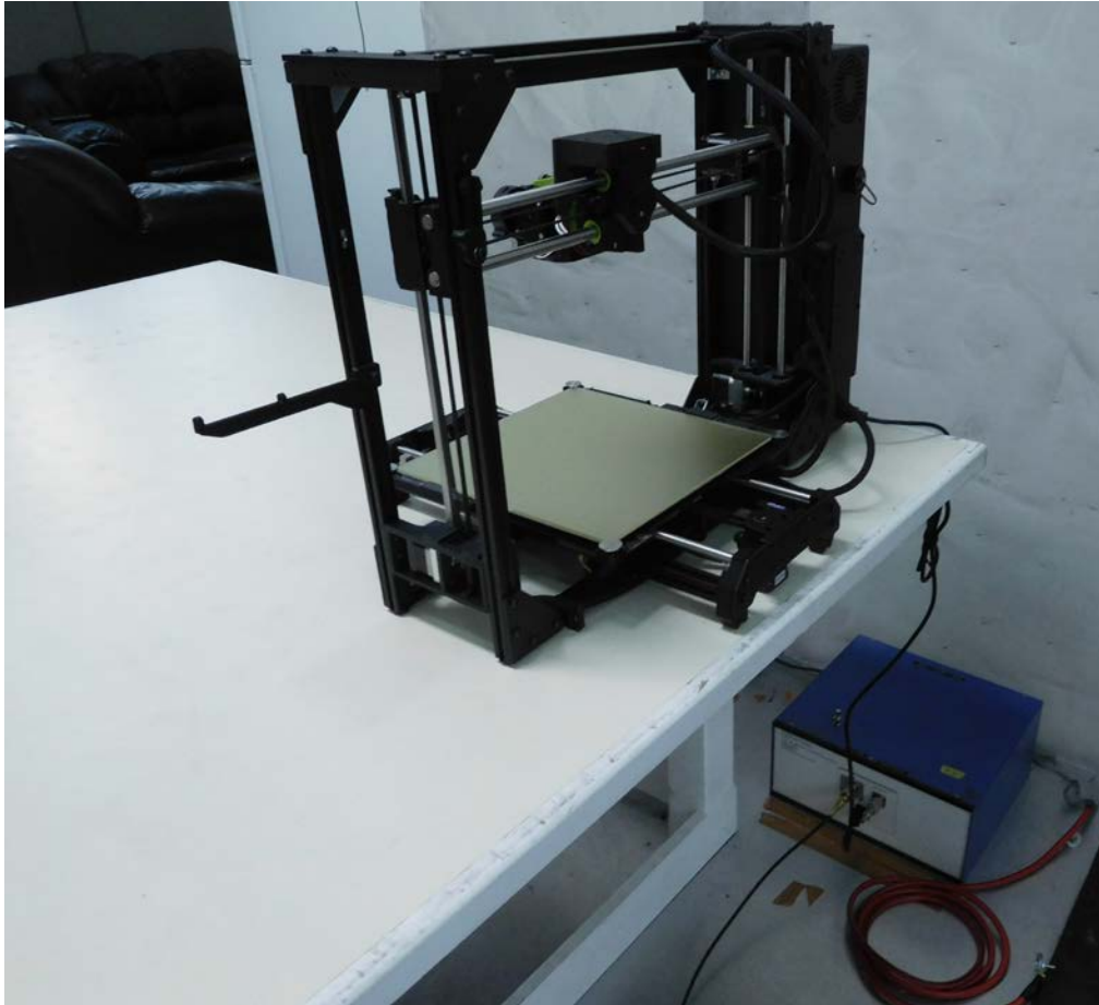
Conducted emissions test setup – running from sd card
