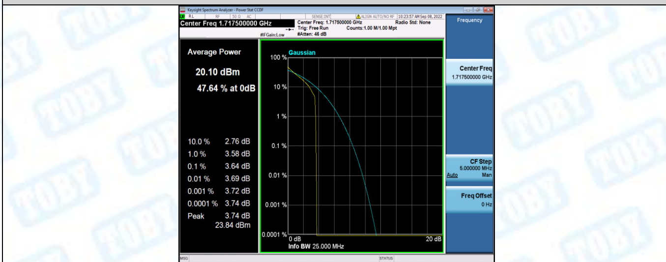
Band66-15MHz-QPSK-132047-75RB#0
