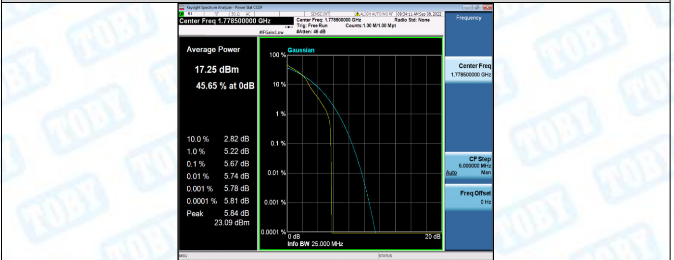
Band66-3MHz-16QAM-132657-15RB#0
