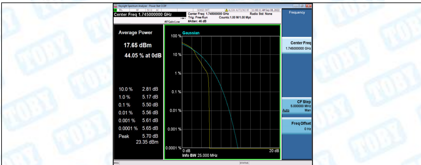
Band66-20MHz-16QAM-132322-100RB#0
