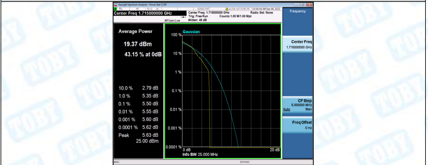
Band66-10MHz-16QAM-132022-50RB#0
