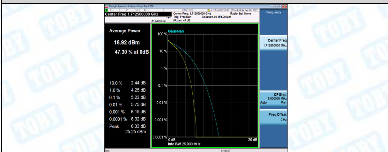
Band66-5MHz-QPSK-132322-1RB#0
