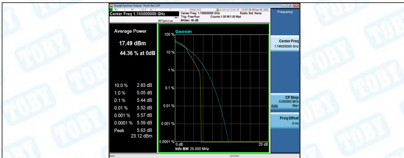
Band66-10MHz-16QAM-132322-50RB#0
