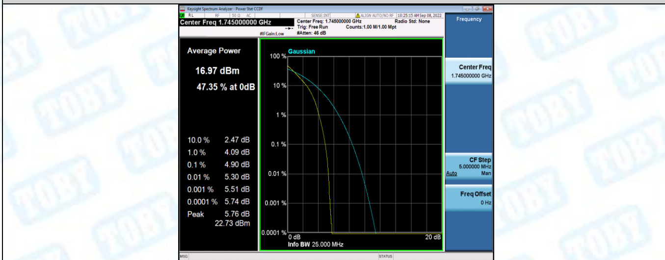
Band66-15MHz-QPSK-132597-1RB#0
