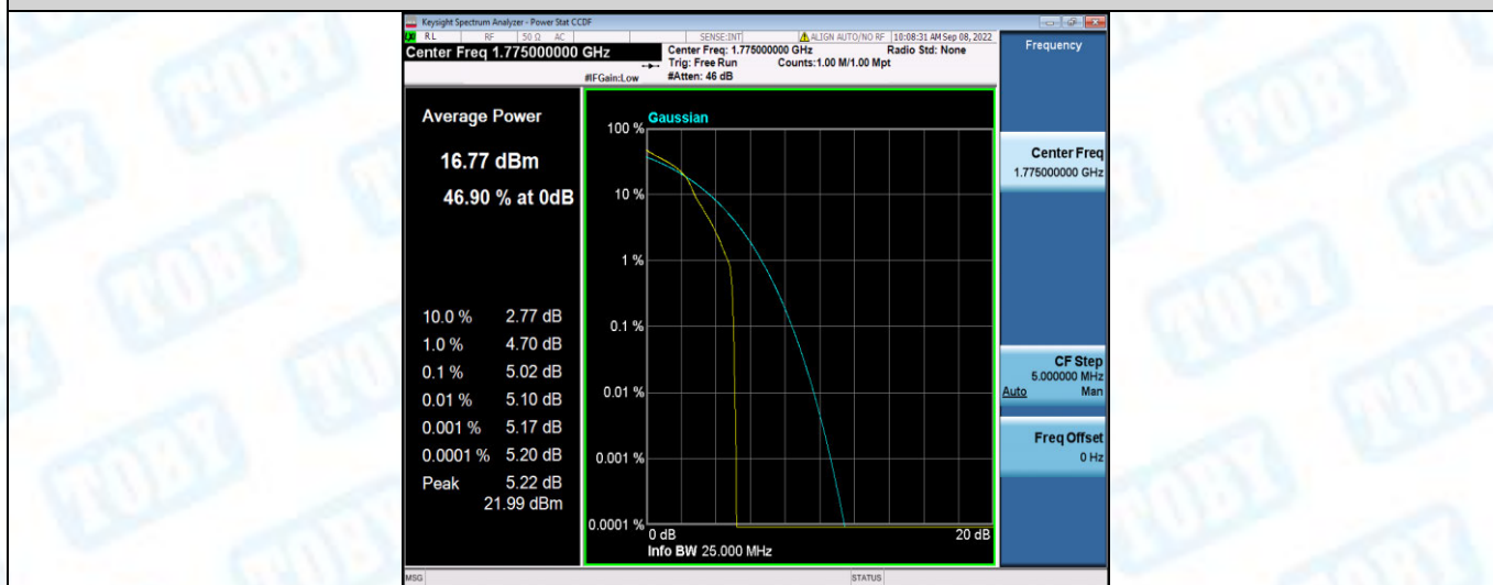
Band66-10MHz-16QAM-132622-50RB#0
