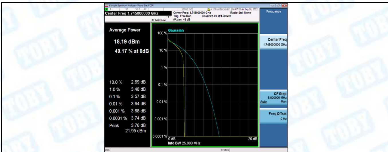
Band66-10MHz-QPSK-132322-50RB#0
