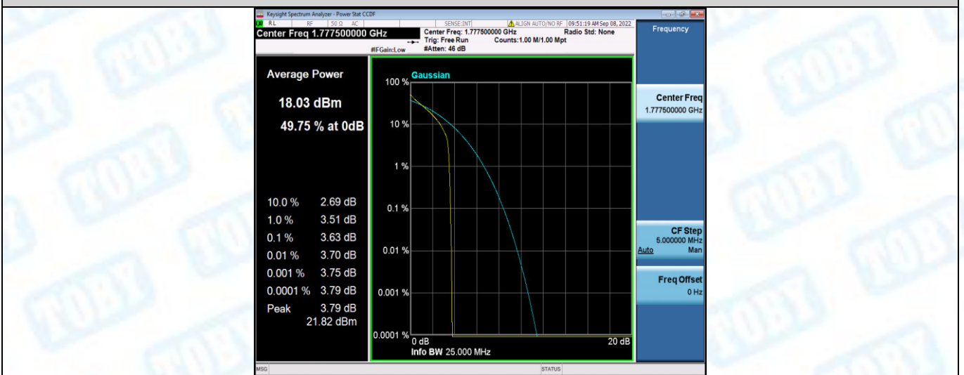
Band66-5MHz-QPSK-132647-25RB#0
