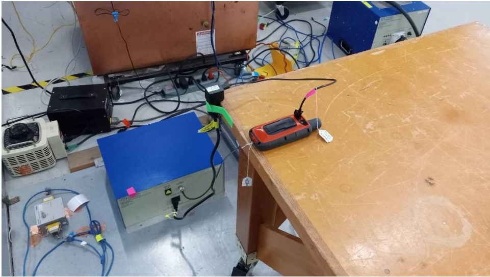
Conducted emissions test setup
