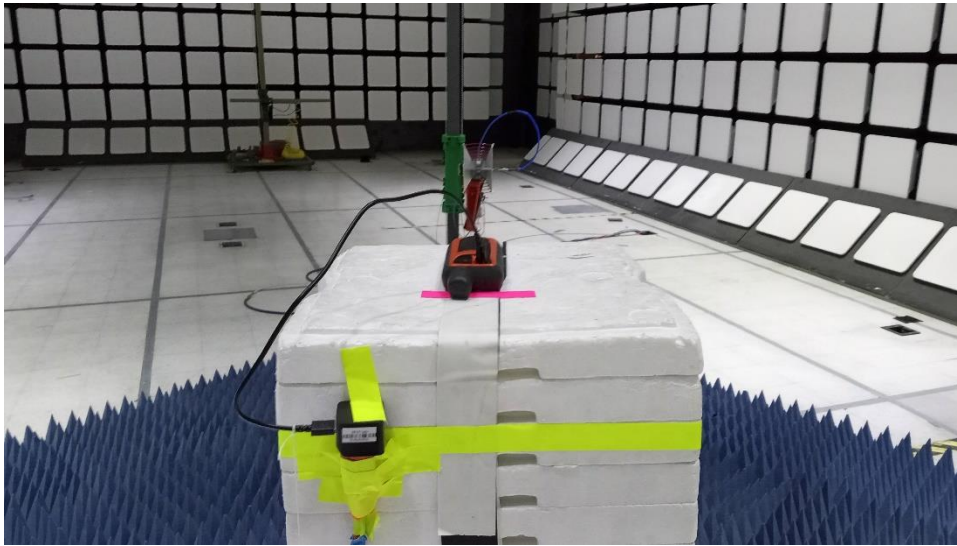
1 – 26 GHz Test Setup
