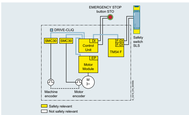
SLS integrated safety technology using fail-safe inputs
