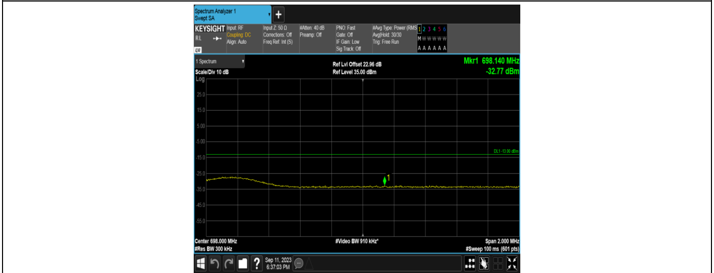
Band71-15MHz-16QAM-133397-1RB#0
