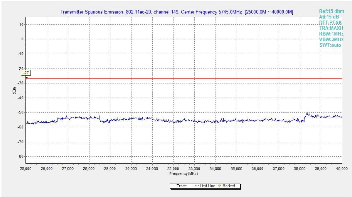
Fig. 42 Conducted Spurious Emission (802.11ac20, Ch149 , 25 GHz ~ 40 GHz)
