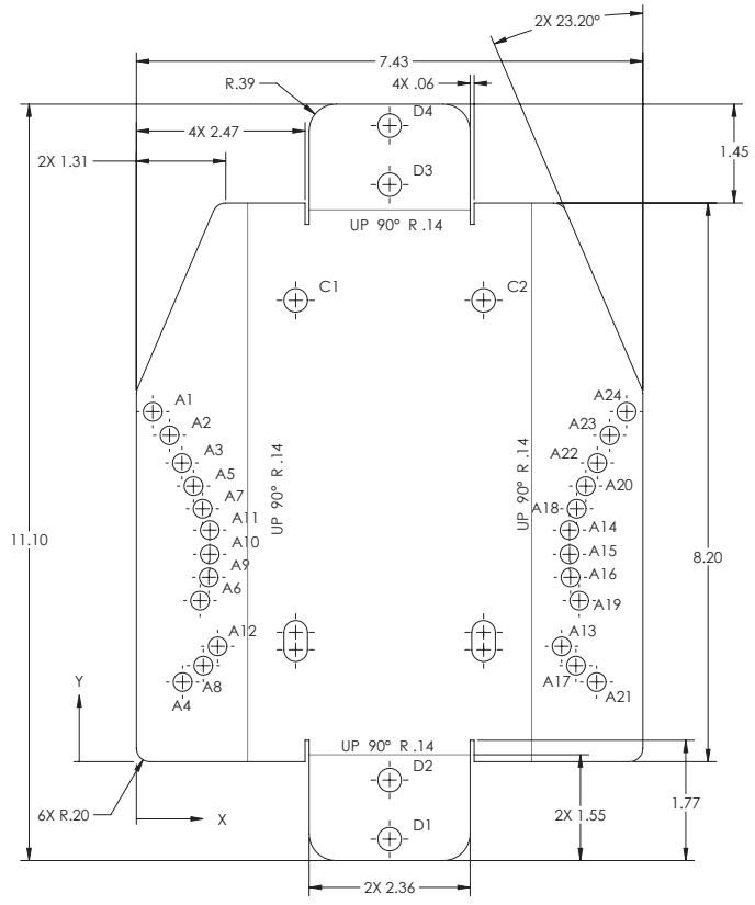
FLAT PATTERN ⑨
