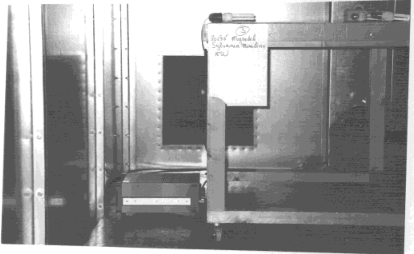
7.1 Conducted emission measurement setup in shielded room
