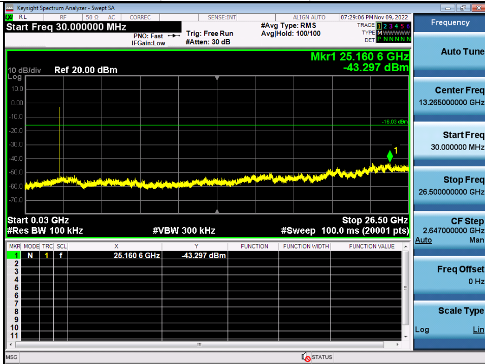
2_Spurious_Emission_BLE_1Mbps_2402
