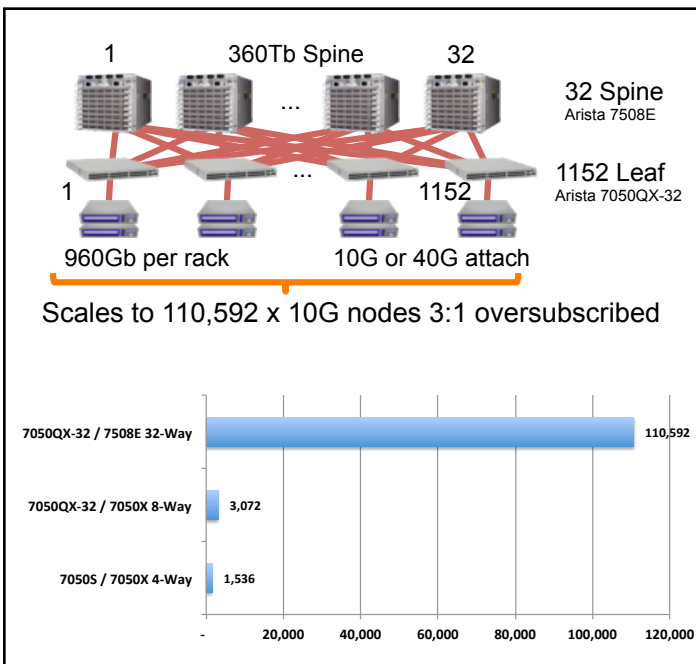
Arista Leaf-Spine Design with L3
