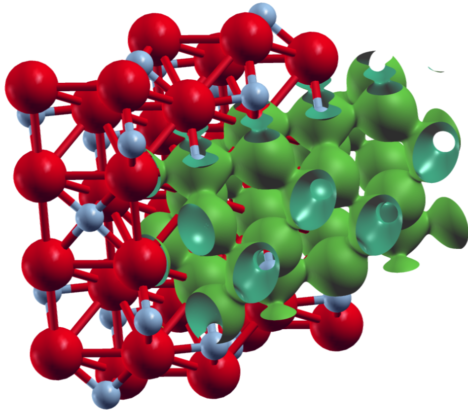
Figure 4.5: XCrySDen plot of an isosurface for the total charge density for Fe 2 N.
