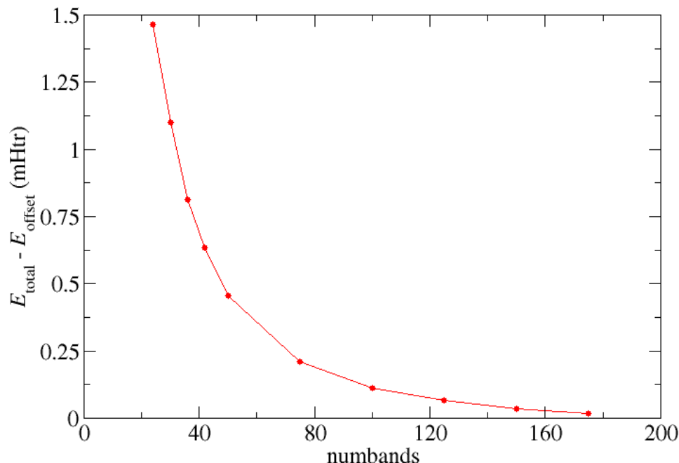
Figure 5.13: numbands convergence for SOC calculations on Pb.
