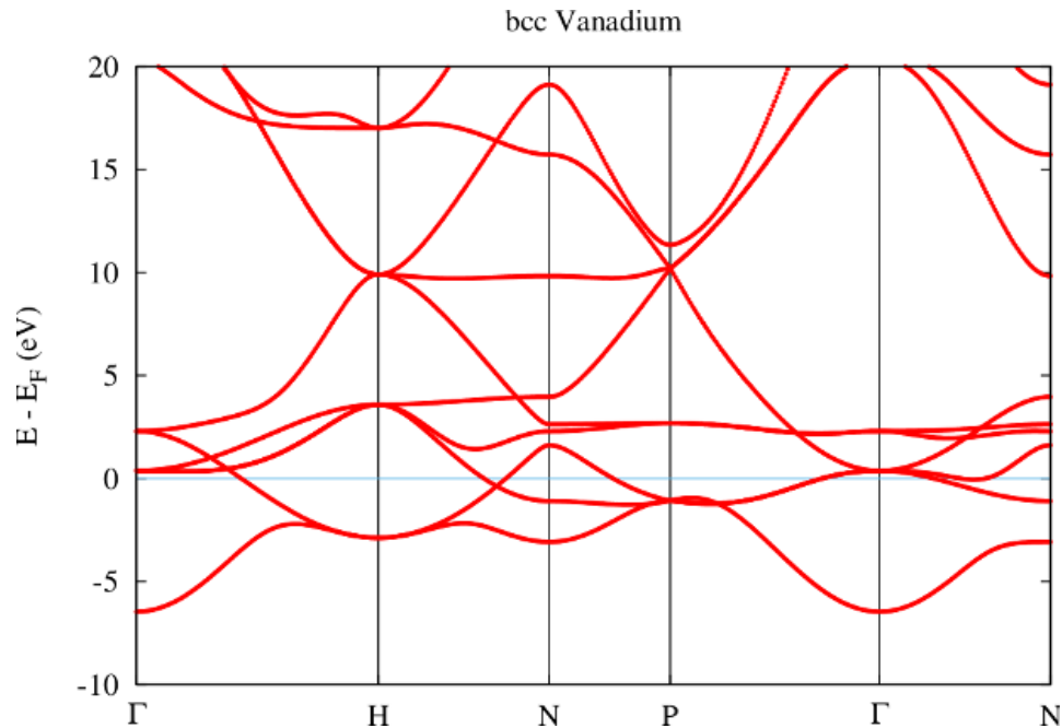
Figure 5.8: No more ghost band in Vanadium. R_{MT} = 2.16 a_0 , core electrons reaching out of MT: 0.012, semicore LO for 3p state
