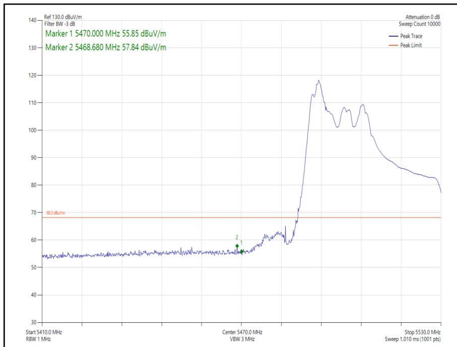
Figure 218 - 802. 11ax HE40 SDM, Cores 0-1, 26-0 - 5510 MHz Band Edge Frequency 5470 MHz
