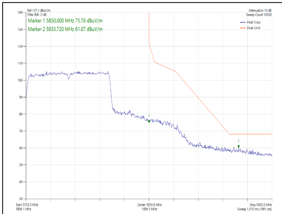
Figure 246 - 802.11ac VHT80 Core 1 - 5775 MHz Band Edge Frequency 5850 MHz
