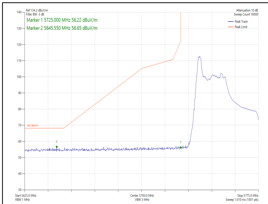
Figure 209 - 802.11ax HE40, Core 1, 26-0 - 5755 MHz Band Edge Frequency 5725 MHz
