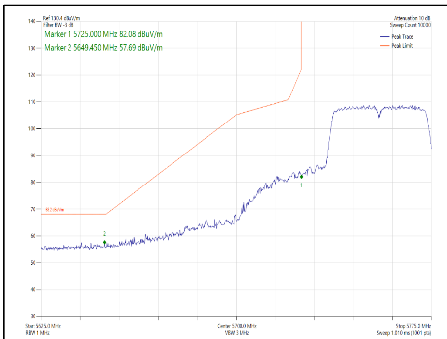
Figure 207 - 802.11n HT40, Core 1 - 5755 MHz Band Edge Frequency 5725 MHz
