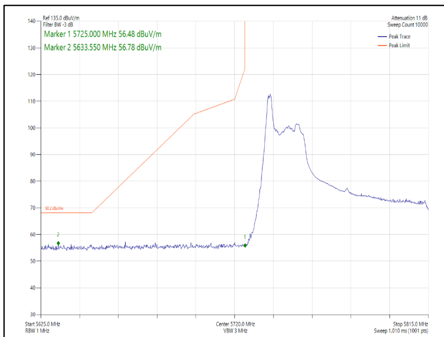
Figure 245 - 802.11ax HE80 Core 1 26-0 - 5775 MHz Band Edge Frequency 5725 MHz
