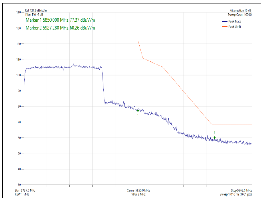
Figure 247 - 802.11ax HE80 Core 1 SU - 5775 MHz Band Edge Frequency 5850 MHz
