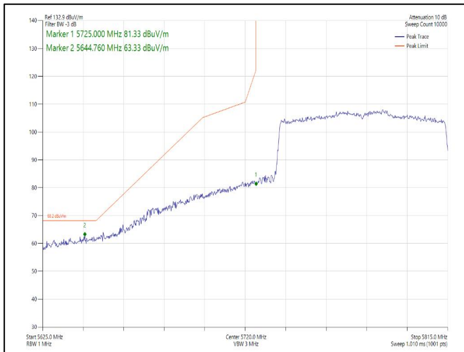
Figure 244 - 802.11ax HE80 Core 1 SU - 5775 MHz Band Edge Frequency 5725 MHz
