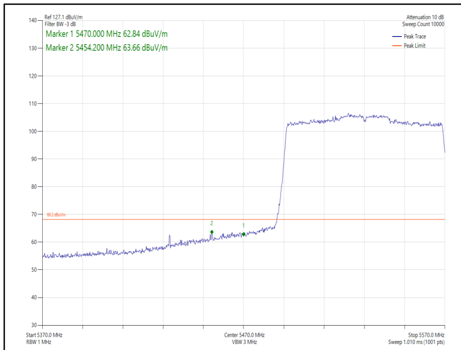
Figure 238 - 802.11ax HE80 Core 1 SU - 5530 MHz Band Edge Frequency 5470 MHz
