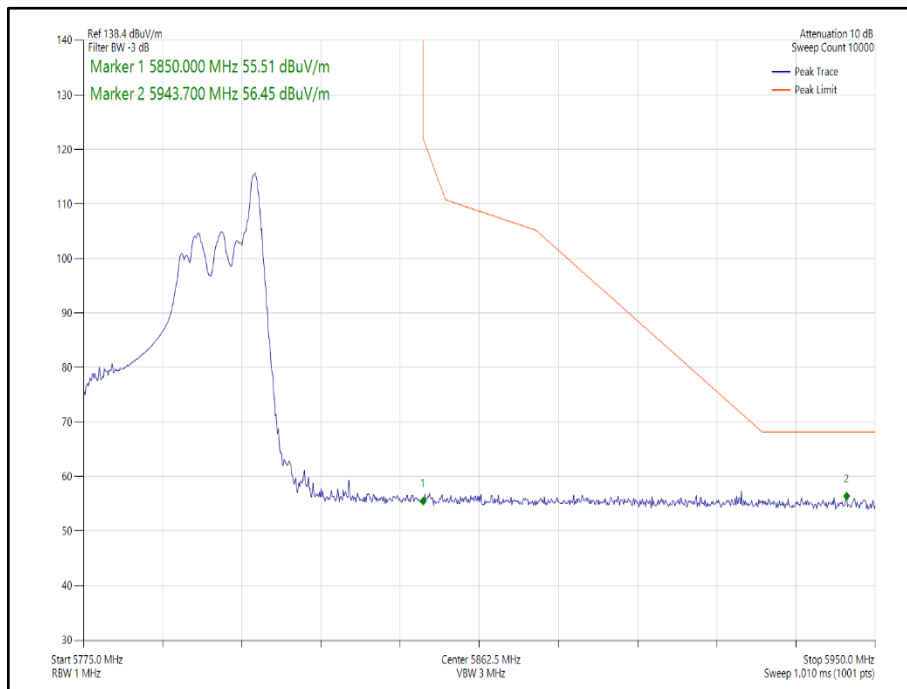
Figure 234 - 802.11ax HE40 CDD, Cores 0-1, 26-17 - 5795 MHz Band Edge Frequency 5850 MHz
