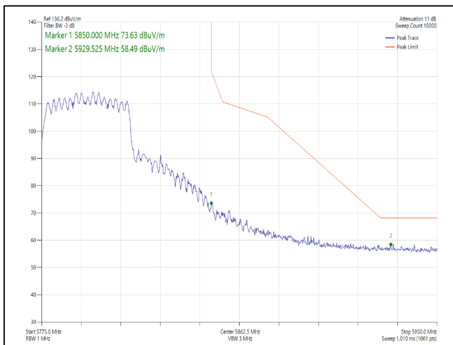
Figure 233 - 802.11ax HE40 CDD, Cores 0-1, SU - 5795 MHz Band Edge Frequency 5850 MHz
