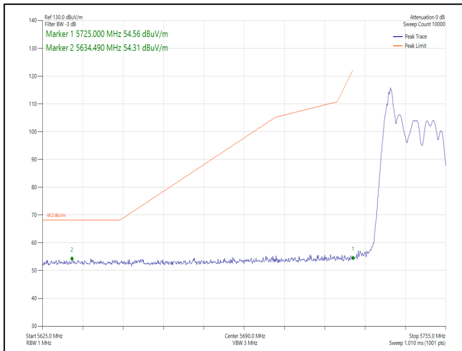
Figure 194 - 802.11x HE20 SDM, Cores 0-1, 26-0 - 5745 MHz Band Edge Frequency 5725 MHz
