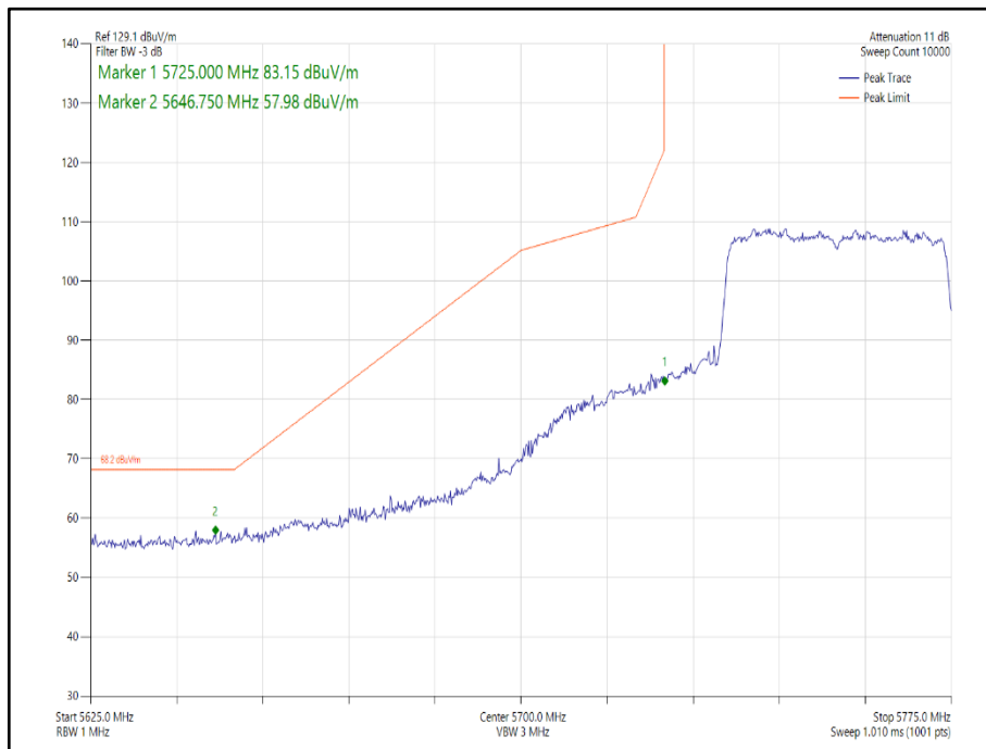
Figure 208 - 802.11ax HE40, Core 1, SU - 5755 MHz Band Edge Frequency 5725 MHz
