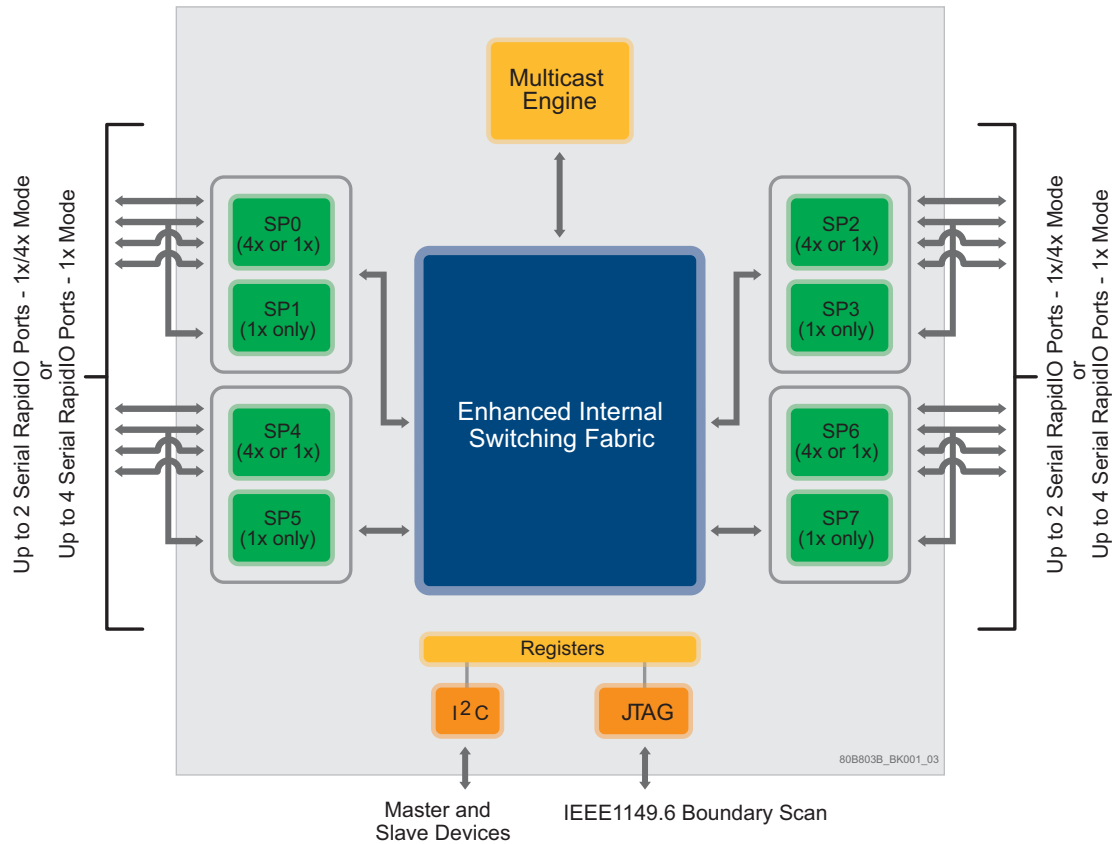
Figure 1: Block Diagram
