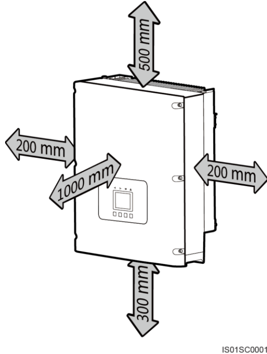
Figure 1-4 Minimum installation clearance
