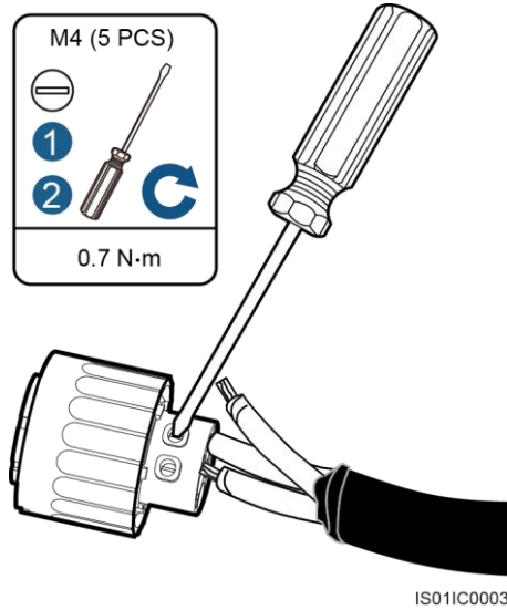
Figure 1-22 Connecting an AC output power cable (5)
