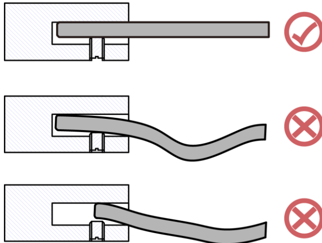
Figure 1-23 Connecting an AC output power cable (6)
