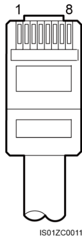
Figure 1-30 Connecting a communications cable (1)
