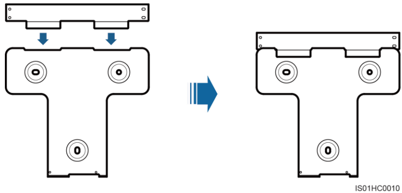
Figure 1-14 Mounting the SUN2000 on the rear panel (rear view)
