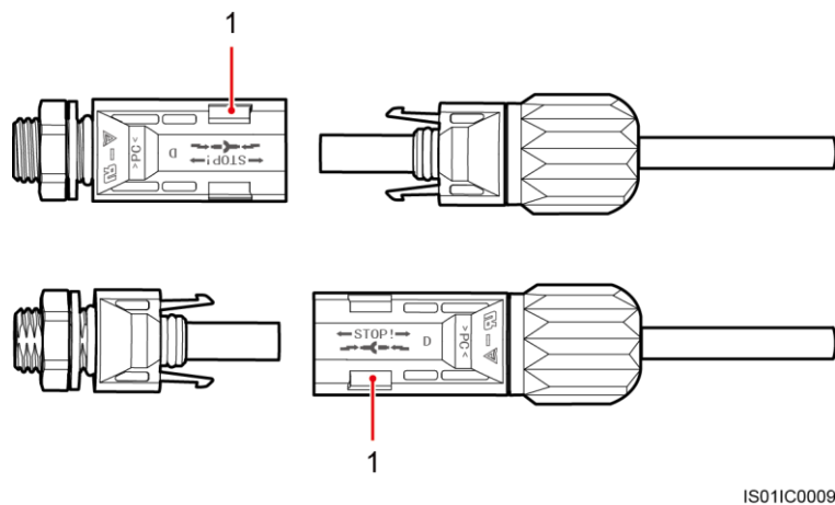
Figure 1-29 Connecting DC input power cables (3)
