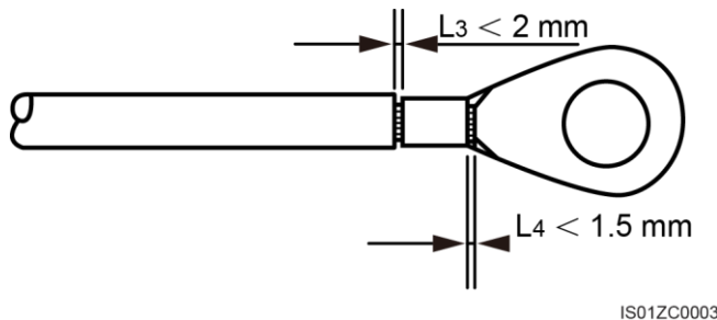
Figure 1-17 Preparing a ground cable (2)
