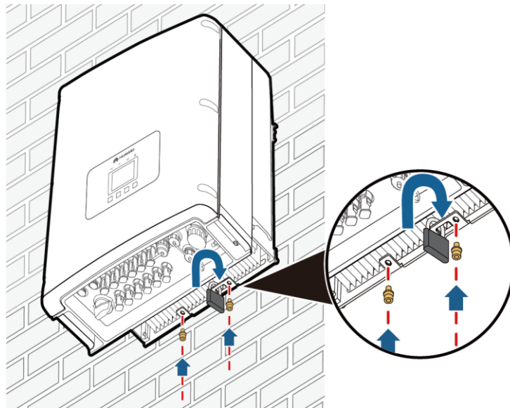
Figure 1-15 Tightening hexagon screws
