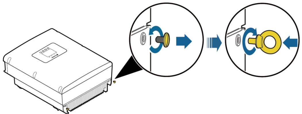
Figure 1-11 Installing lifting eyes
