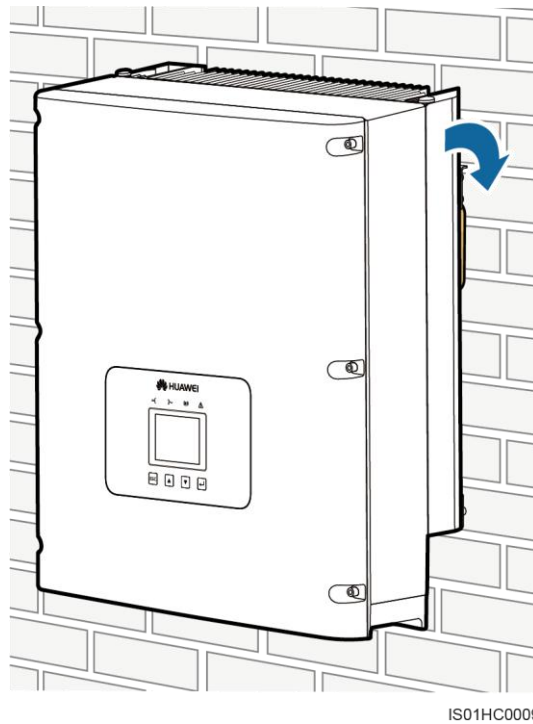
Figure 1-13 Mounting the SUN2000 on the rear panel (front view)
