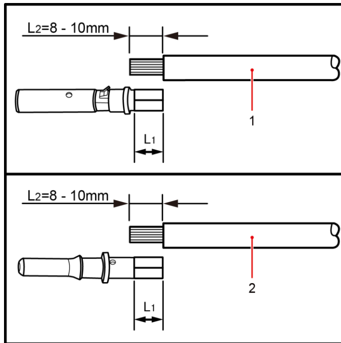
Figure 1-27 Connecting DC input power cables (1)
