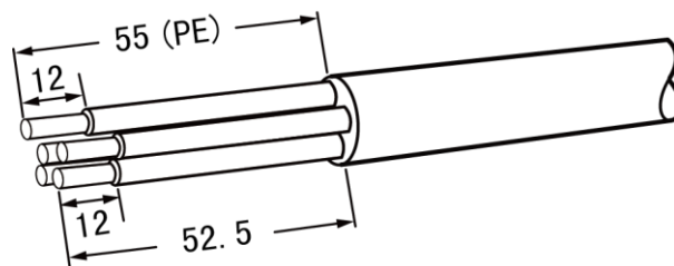
Figure 1-18 Connecting an AC output power cable (1) (unit: mm)
