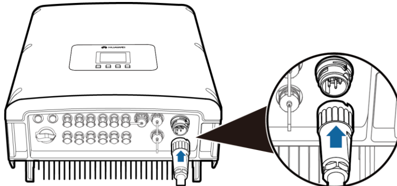
Figure 1-26 Connecting an AC output power cable (9)
