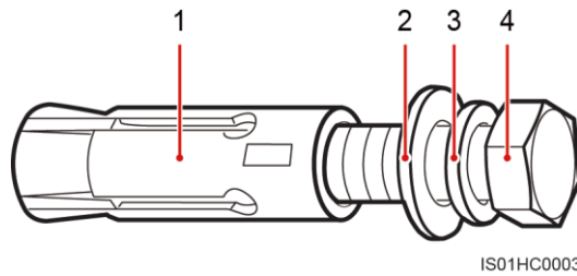
Figure 1-7 Expansion bolt composition
