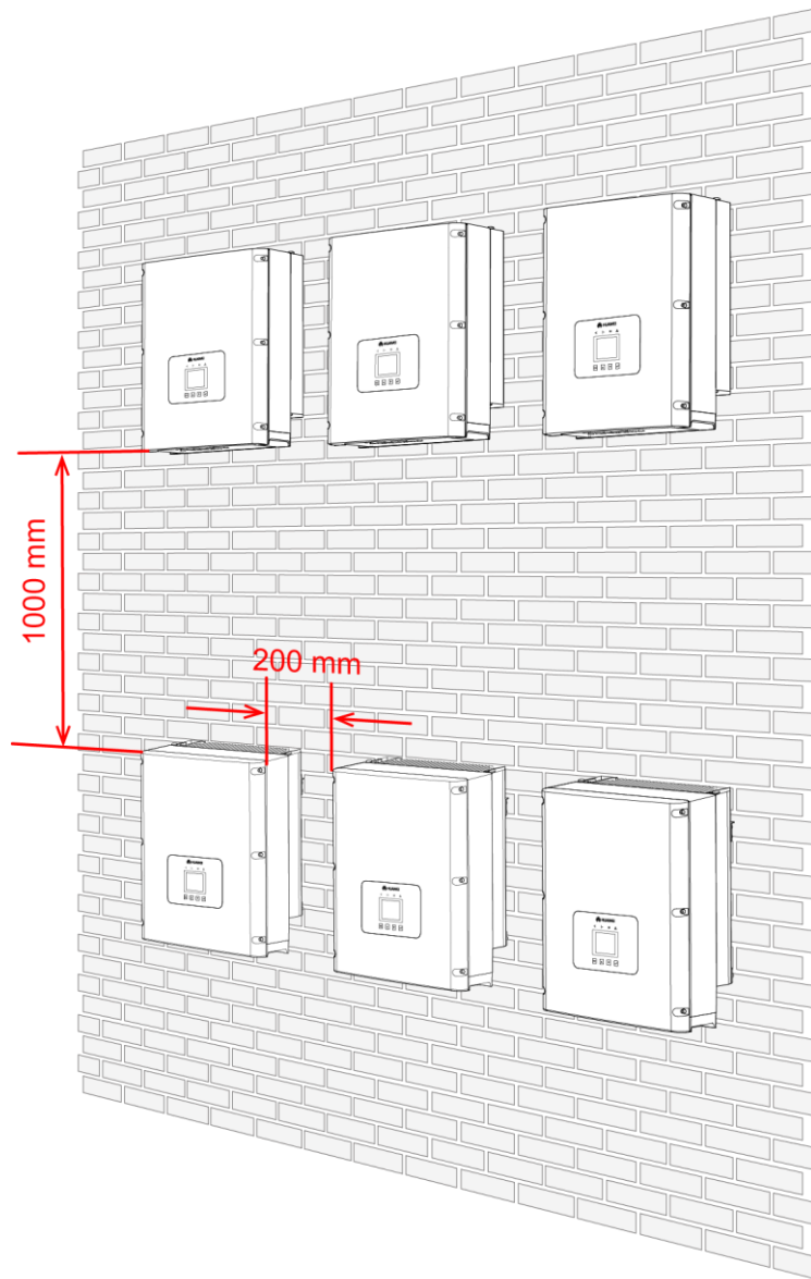
Figure 1-6 Stacked installation mode
