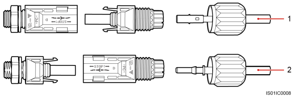
Figure 1-28 Connecting DC input power cables (2)
