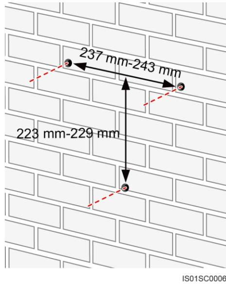
Figure 1-3 Hole positions and dimensions
