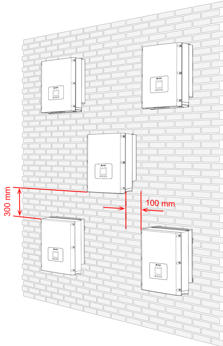
Figure 1-5 Triangle installation mode
