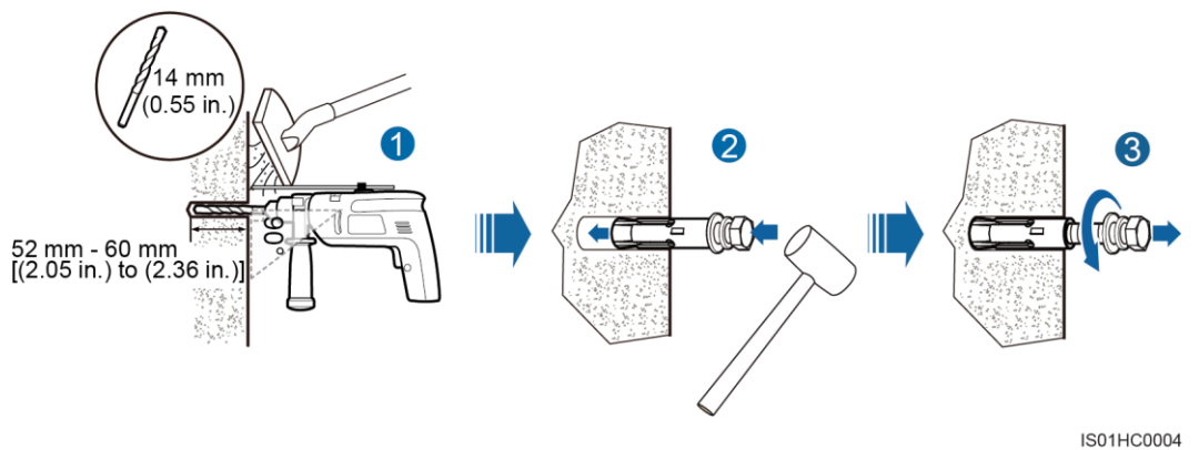
Figure 1-8 Drilling a hole and installing an expansion bolt
