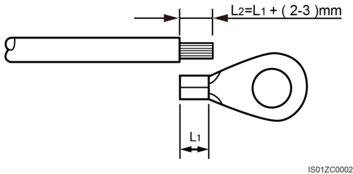
Figure 1-16 Preparing a ground cable (1)
