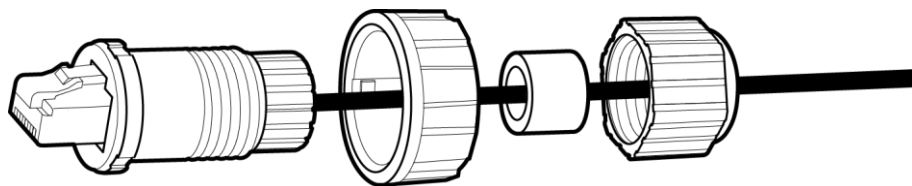
Figure 1-32 Connecting a communications cable (3)
