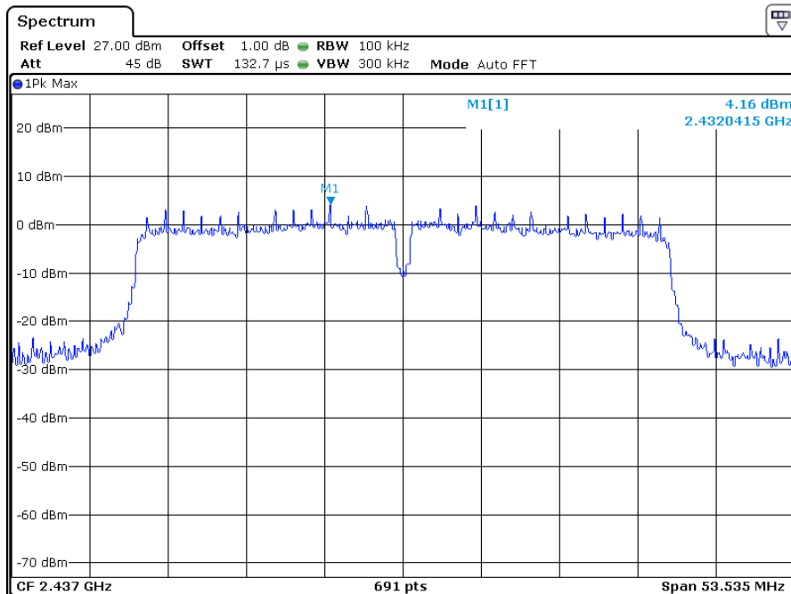
Channel 06 (2437MHz) Reference Level: 4.16dBm
