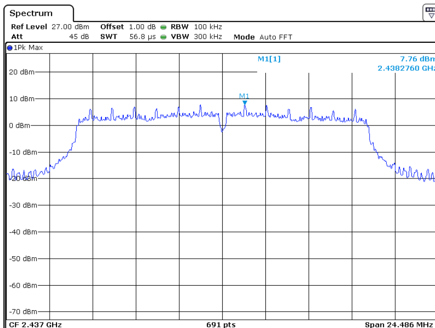
Channel 06 (2437MHz) Reference Level: 7.76dBm
