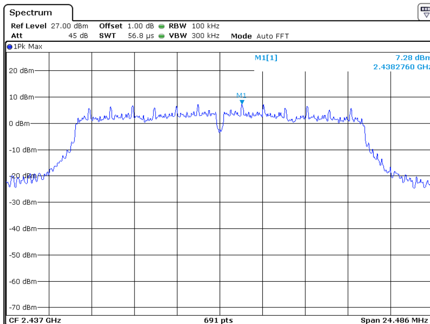
Channel 06 (2437MHz) Reference Level:7.28dBm
