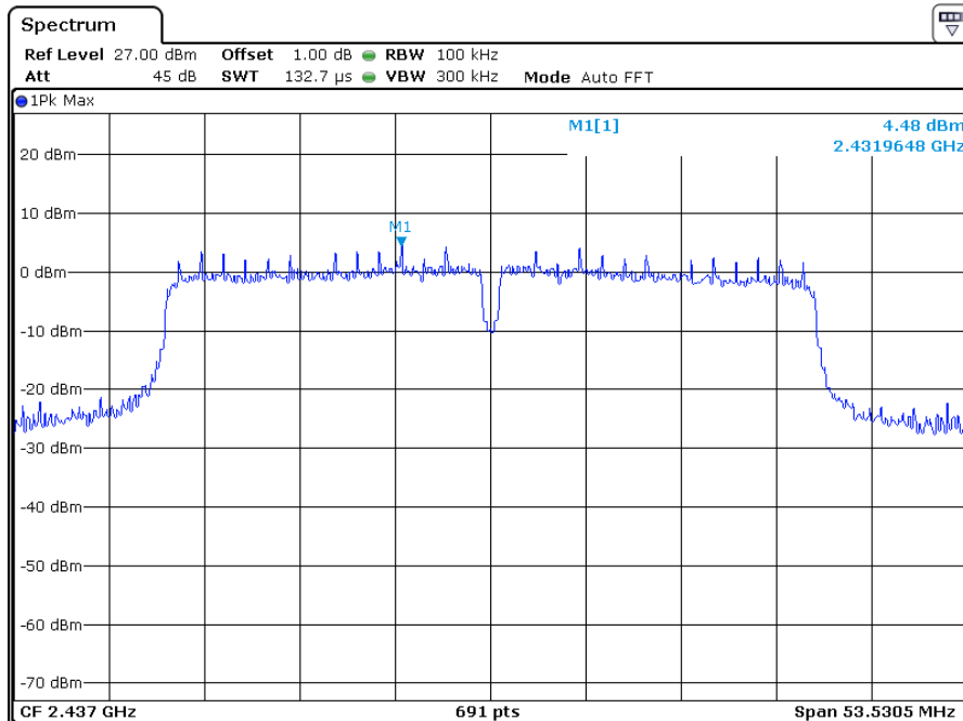
Channel 06 (2437MHz) Reference Level: 4.48dBm
