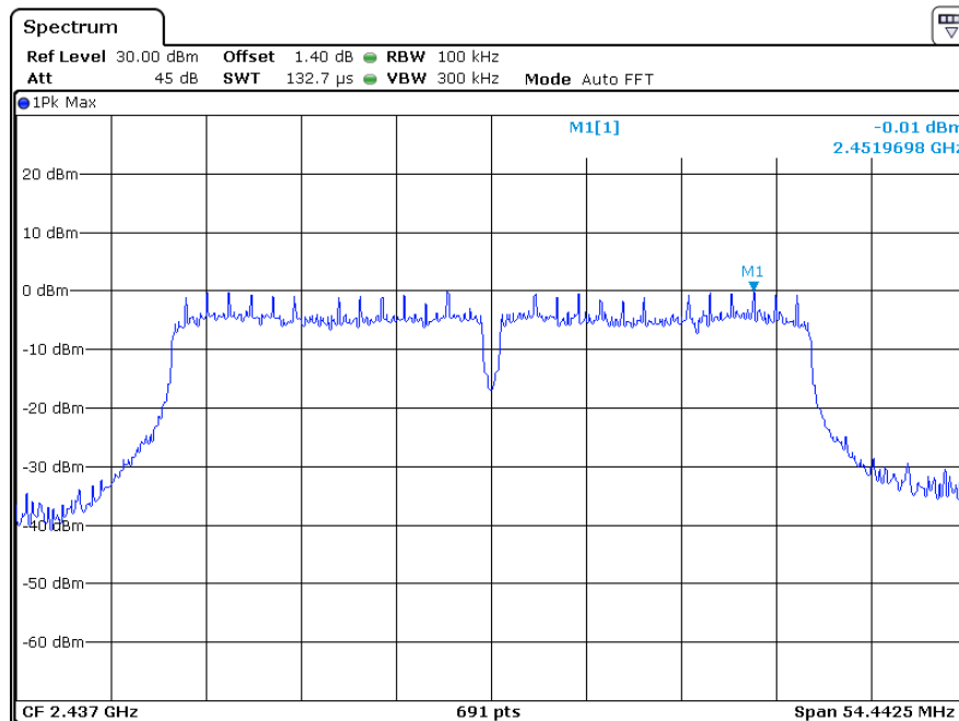
Channel 06 (2437MHz) Reference Level: -0.01dBm
