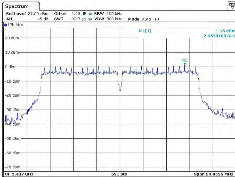
Channel 06 (2437MHz) Reference Level: 1.15dBm
