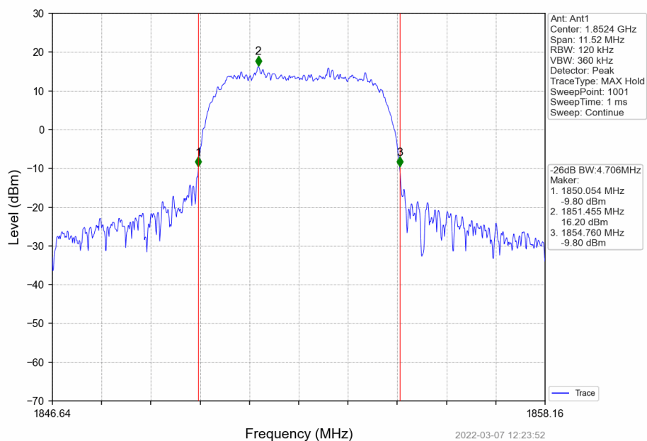
Band2_HSDPA_LCH_1852.4MHz_Subtest 1_NTNV
