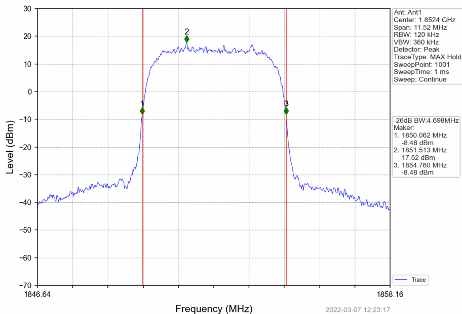
Band2_RMC_LCH_1852.4MHz_12.2kbps RMC_NTNV
