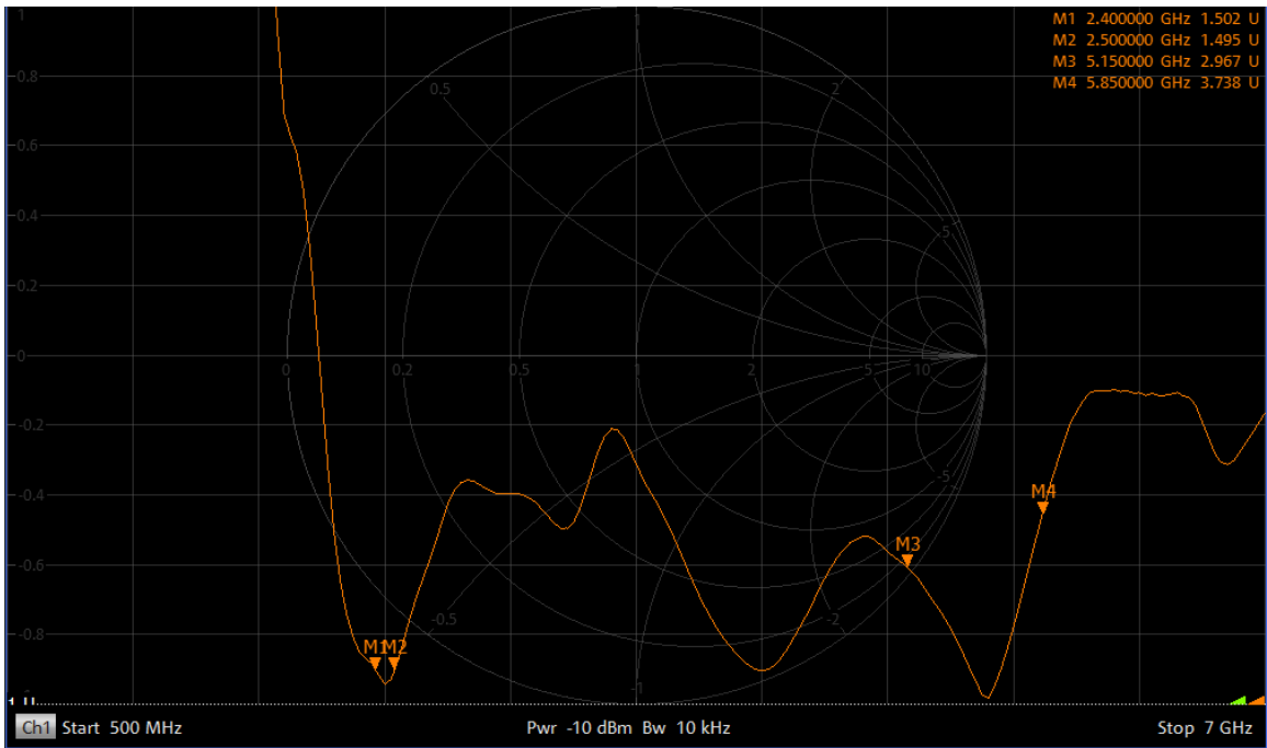
WiFi Antenna
