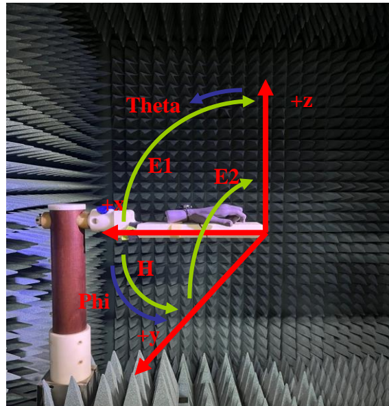
Figure 4: Geometry for SM-R955 for Radiation patterns.
