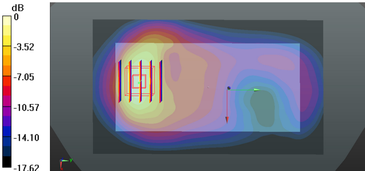
0 dB = 1.01 W/kg
