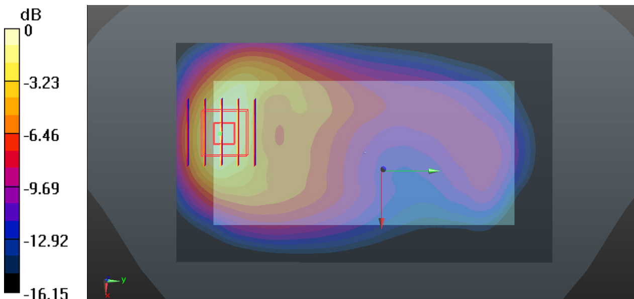
0 dB = 0.626 W/kg
