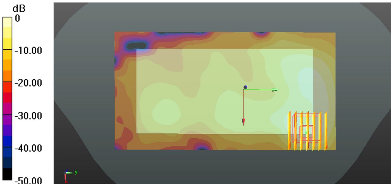
0 dB = 0.0984 W/kg
