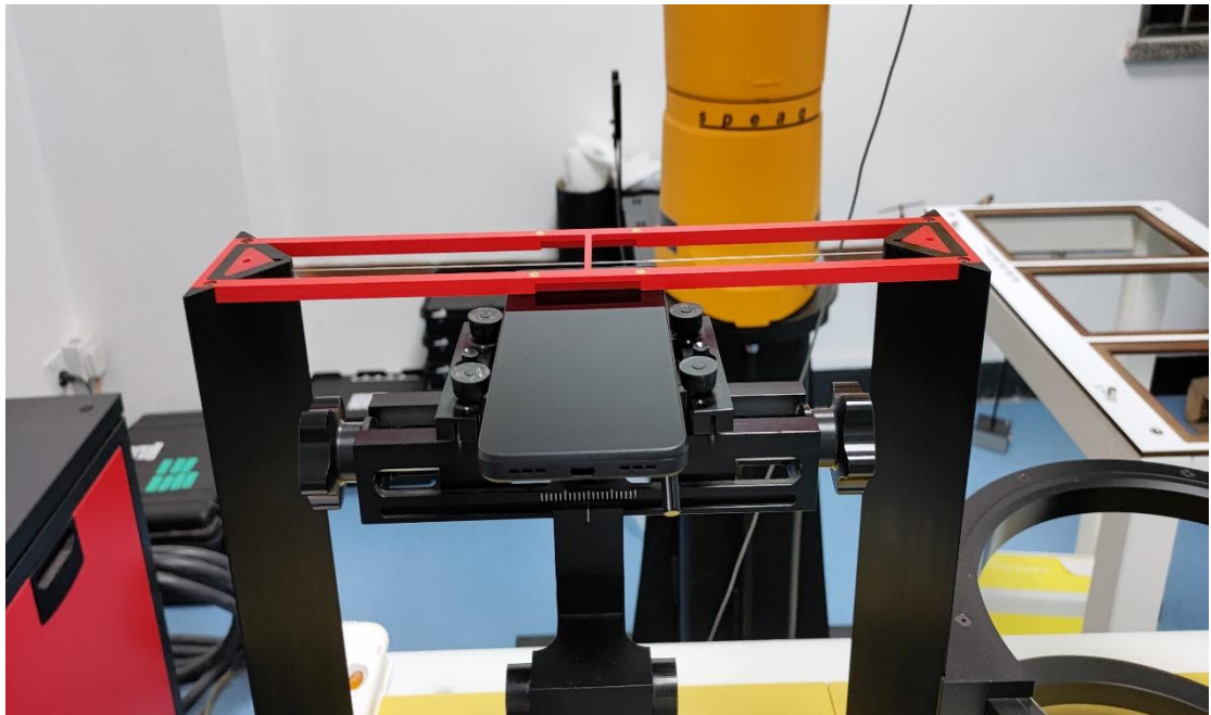
Picture 2: EUT Positioning for RF/T-coil
