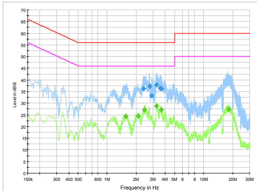
Fig.126. AC Powerline Conducted Emission-idle-ch39
