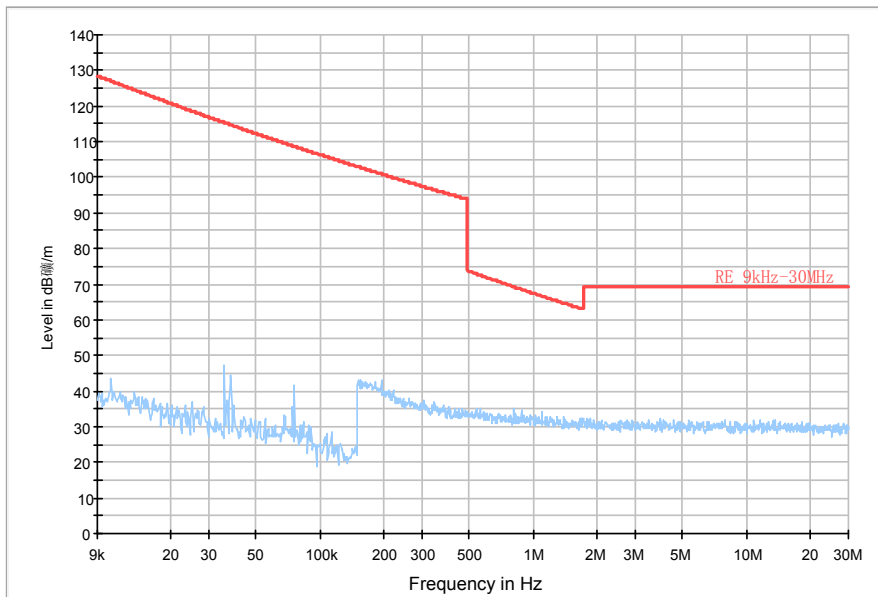
RE 9kHz-30MHz
