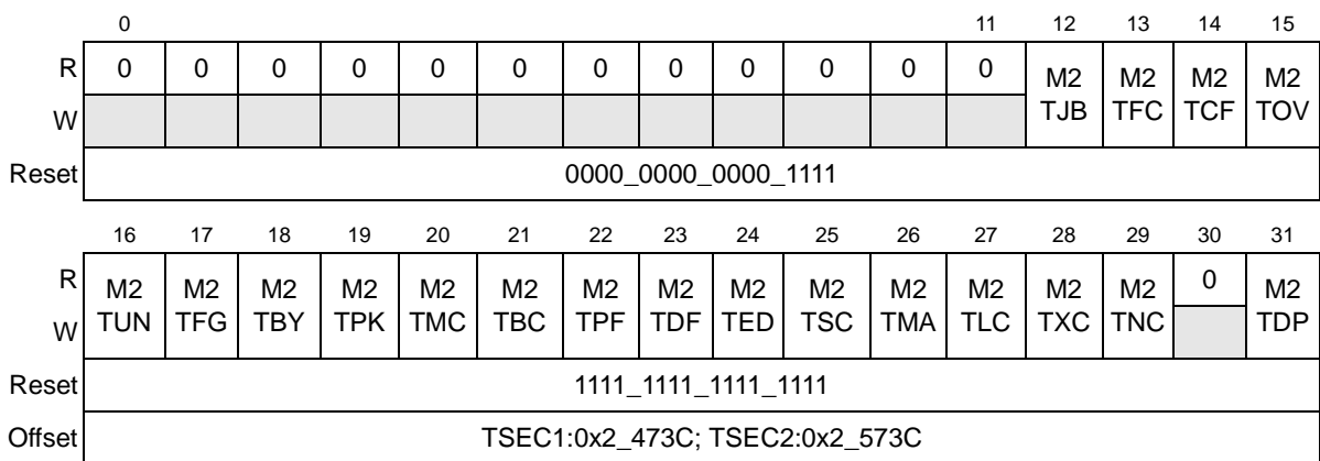
Figure 13-95. Carry Mask Register 2 (CAM2) Register Definition
