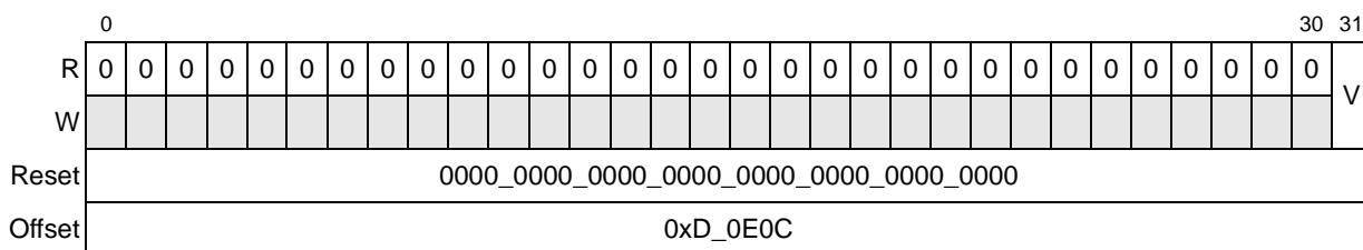
Figure 16-42. Port Error Capture Status Register (PECSR)
