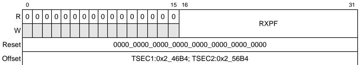
Figure 13-62. Receive Pause Frame Packet Counter Register Definition
