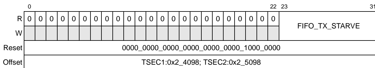
Figure 13-16. FIFO_TX_STARVE Register Definition
