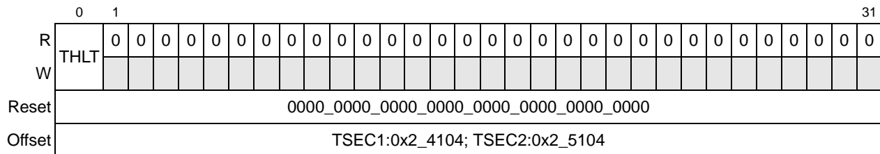
Figure 13-19. TSTAT Register Definition
