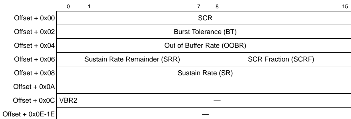
Figure 35-35. Transmit Connection Table Extension (TCTE)—VBR Protocol-Specific
