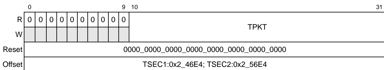
Figure 13-74. Transmit Packet Counter Register Definition
