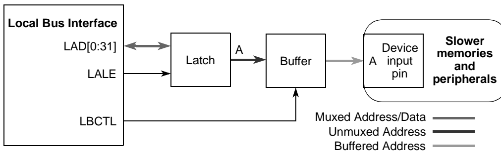
Figure 12-71. GPCM Address Timings
