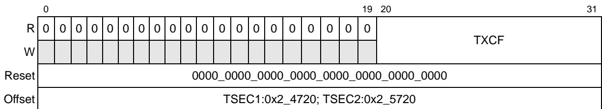
Figure 13-88. Transmit Control Frame Counter Register Definition
