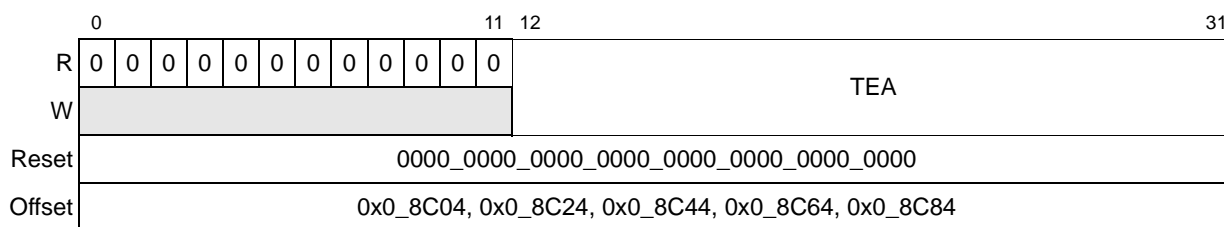
Figure 15-7. PCI/X Outbound Translation Extended Address Registers
