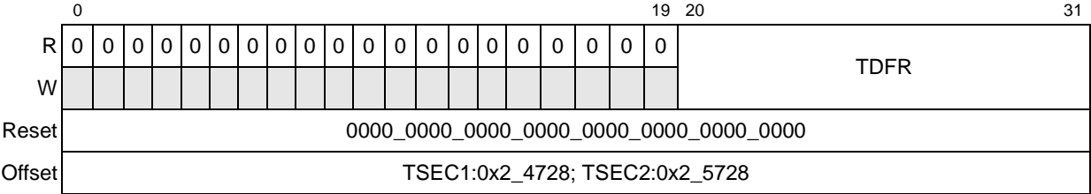
Figure 13-90. Transmit Undersize Frame Counter Register Definition
