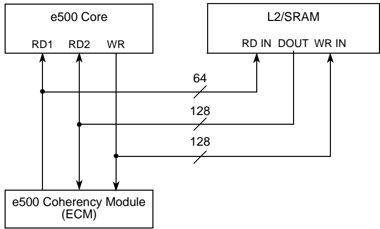
Figure 7-5. Data Bus Connection of CCB
