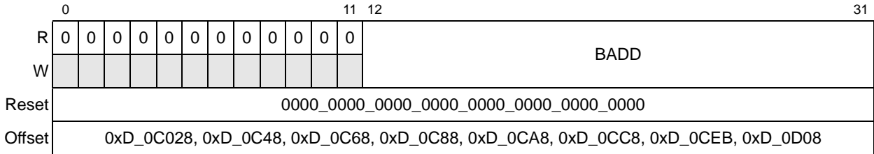
Figure 16-32. RapidIO Outbound Window Base Address Registers 1–8 (ROWBAR n )
