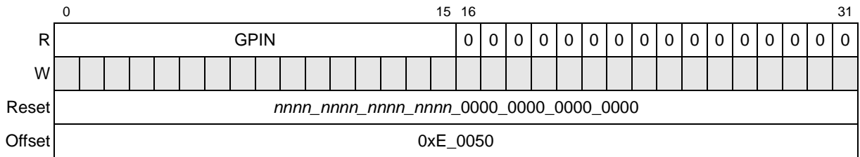
Figure 17-9. General-Purpose Output Data Register (GPINDR)
