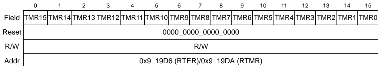
Figure 20-15. RISC Timer Event Register (RTER)/Mask Register (RTMR)
