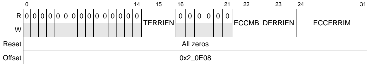
Figure 7-13. L2 Error Injection Mask Control Register (L2ERRINJCTL)
