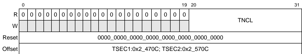
Figure 13-84. Transmit Total Collision Counter Register Definition
