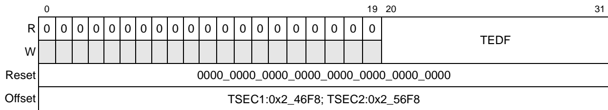
Figure 13-79. Transmit Excessive Deferral Packet Counter Register Definition
