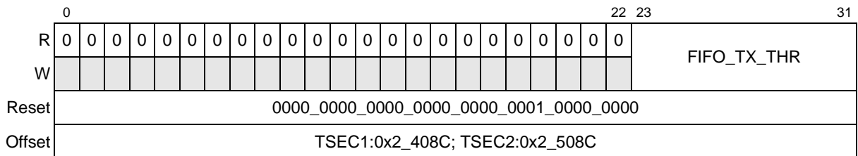
Figure 13-15. FIFO_TX_THR Register Definition
