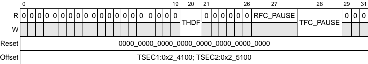
Figure 13-18. TCTRL Register Definition
