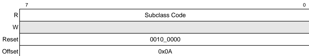
Figure 15-33. PCI Subclass Code Register
