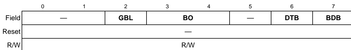
Figure 33-6. TSTATE High Byte
