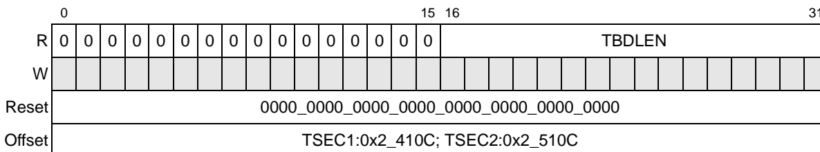
Figure 13-20. TBDLEN Register Definition
