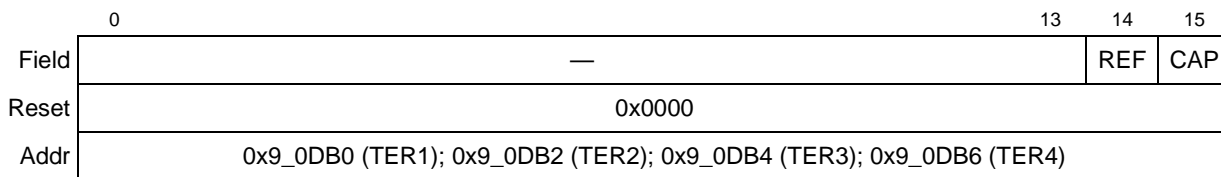
Figure 25-9. Timer Event Registers (TER1–TER4)
