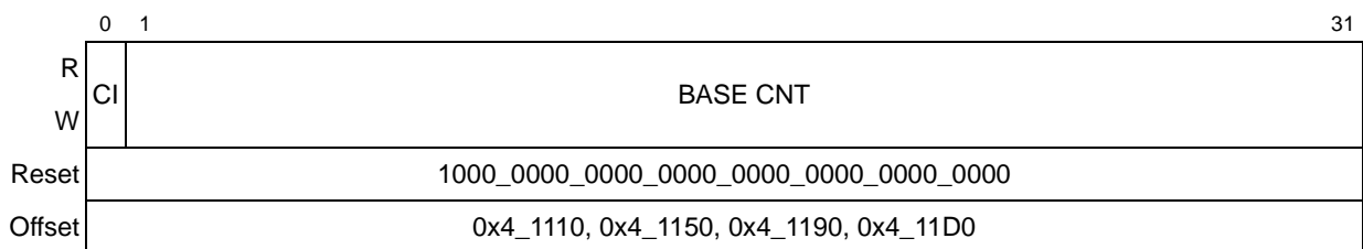
Figure 10-11. Global Timer Base Count Registers (GTBCR n )
