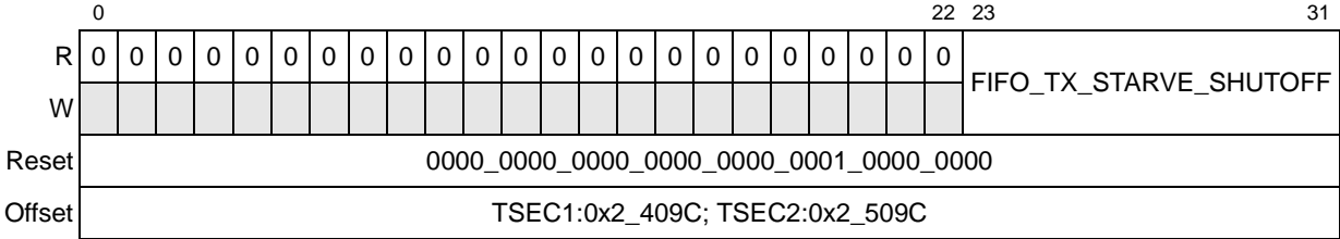
Figure 13-17. FIFO_TX_STARVE_SHUTOFF Register Definition
