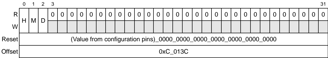
Figure 16-21. Port General Control Command and Status Register (PGCCSR)
