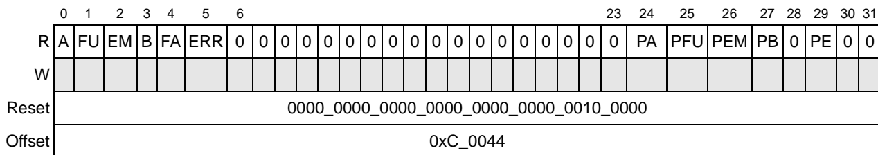
Figure 16-12. Port-Write and Doorbell Command and Status Register (PWDCSR)
