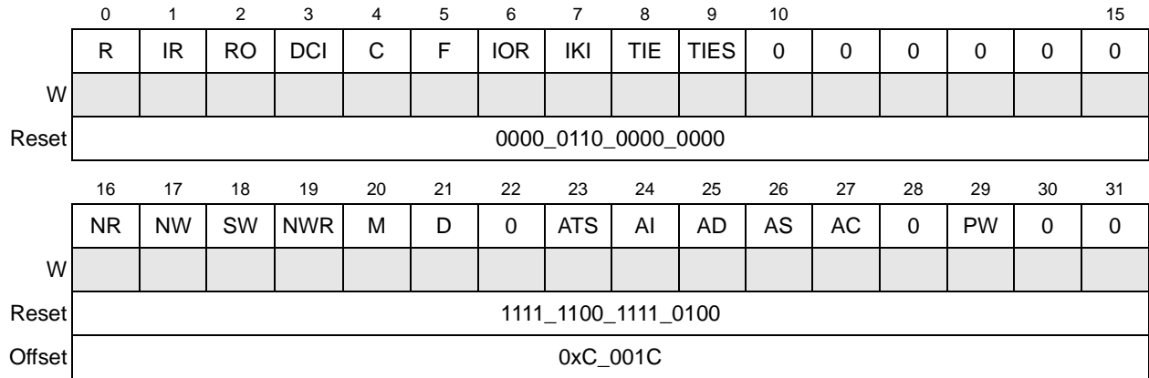
Figure 16-10. Destination Operations Capability Register (DOCAR)
