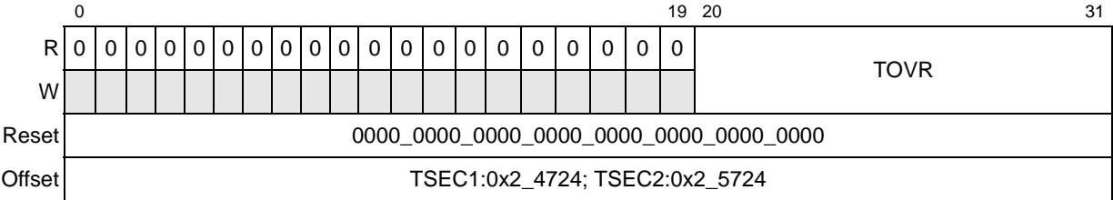
Figure 13-89. Transmit Oversized Frame Counter Register Definition
