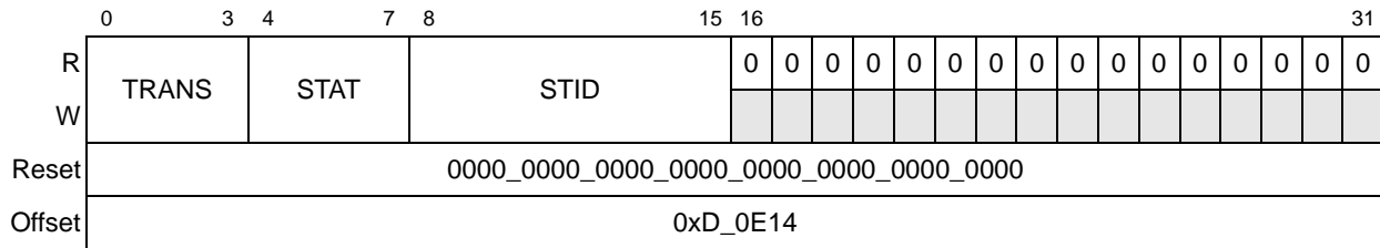
Figure 16-52. Error Packet Capture Register 1 (EPCR1)—Type 13 Packet Format
