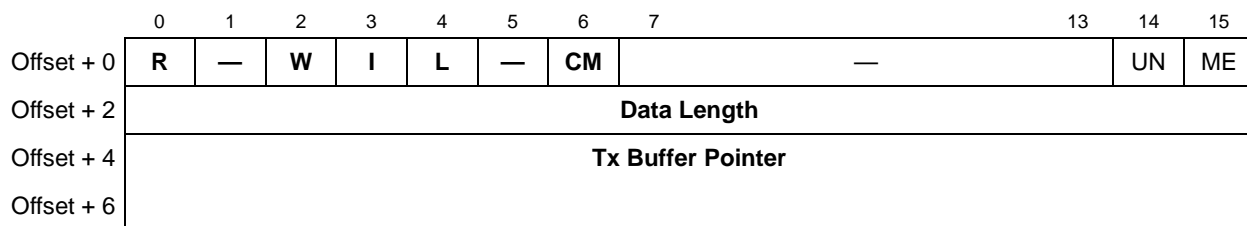
Figure 43-12. SPI TxBD
