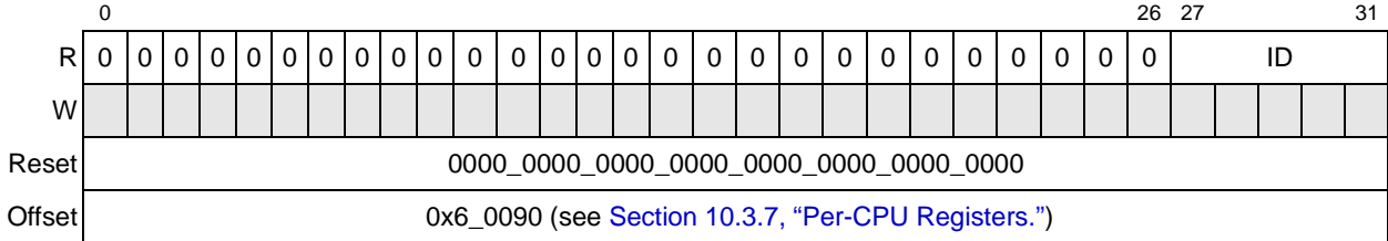
Figure 10-34. Processor Who Am I Register (WHOAMI)
