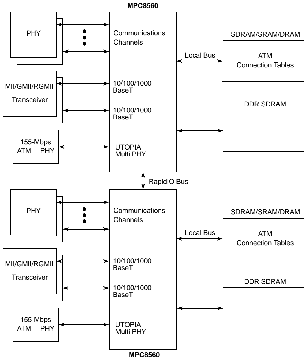
Figure 1-6. High-Performance Communications
