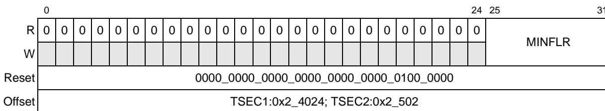
Figure 13-10. MINFLR Register Definition
