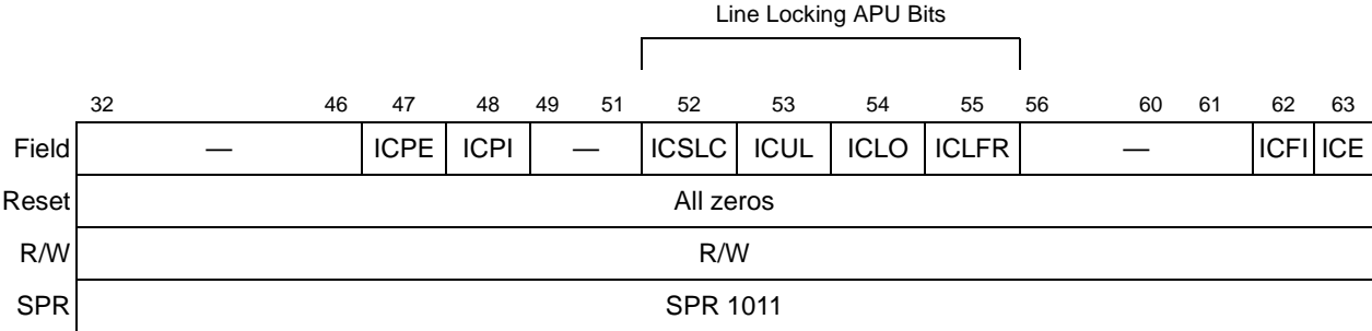
Figure 6-34. L1 Cache Control and Status Register 1 (L1CSR1)
