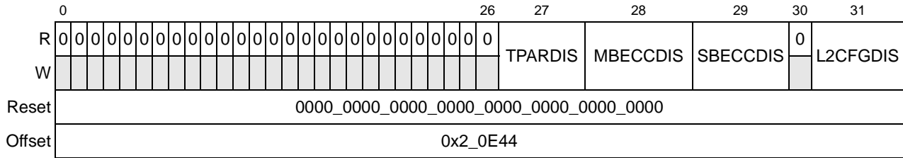
Figure 7-18. L2 Error Disable Register (L2ERRDIS)
