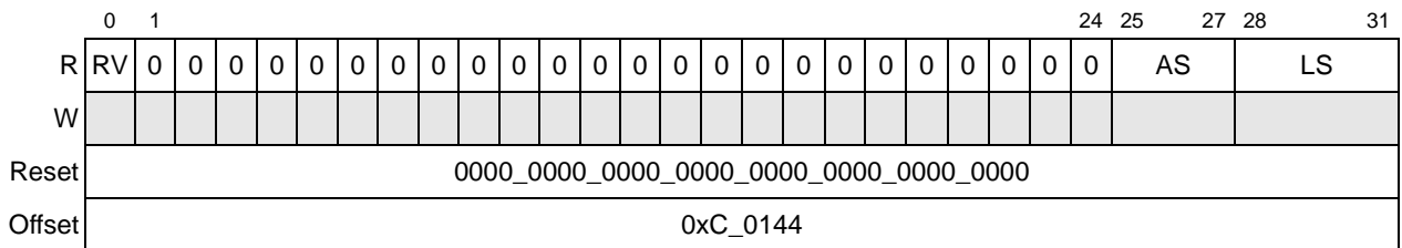
Figure 16-23. Port Link Maintenance Response Command and Status Register (PLMRESPCSR)
