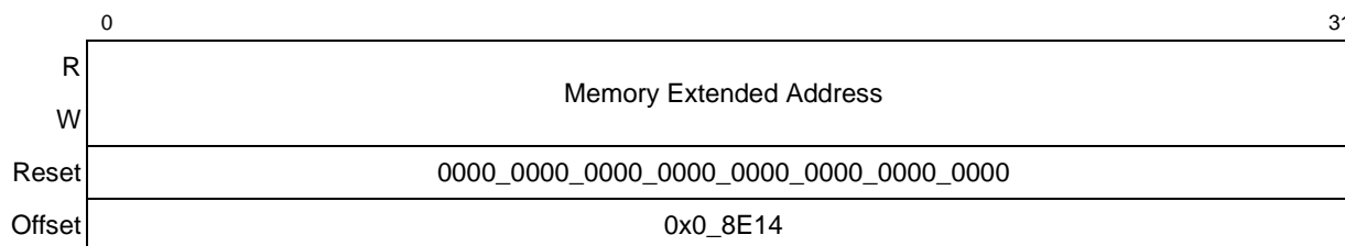
Figure 15-20. PCI/X Error Extended Address Capture Register (ERR_EXT_ADDR)
