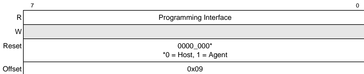
Figure 15-32. PCI Bus Programming Interface Register
