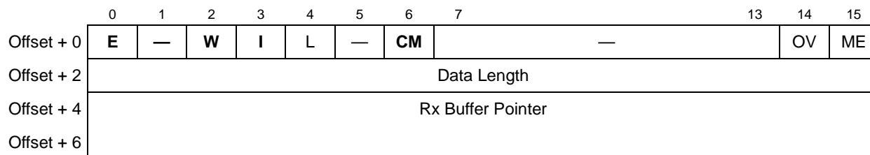
Figure 43-11. SPI RxBD
