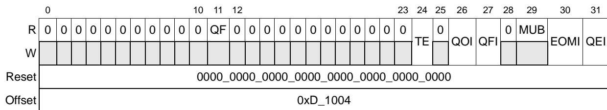
Figure 16-63. Outbound Status Register (OSR)
