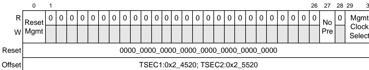
Figure 13-40. MII Management Configuration Register Definition
