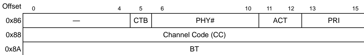
Figure 35-68. COMM_INFO Field
