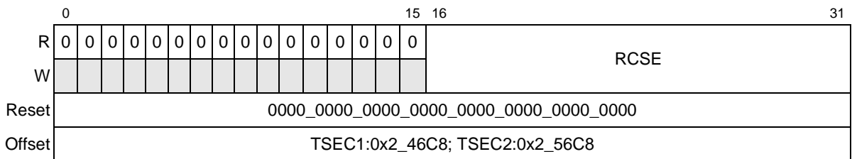
Figure 13-67. Receive Carrier Sense Error Counter Register Definition
