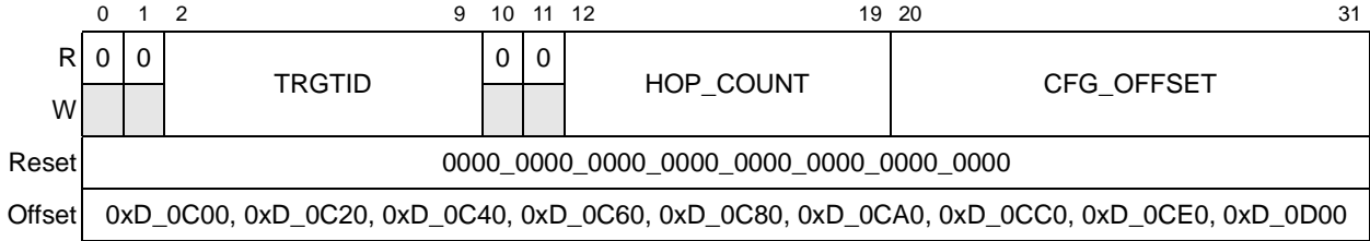
Figure 16-31. RapidIO Outbound Window Translation Address Registers 0–8 for Maintenance Transactions (ROWTAR n )
