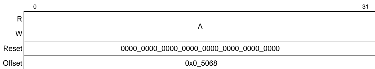
Figure 12-6. UPM Memory Address Register (MAR)
