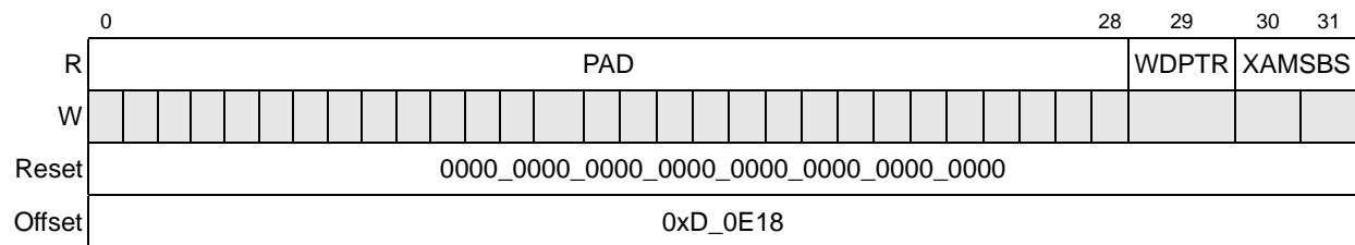
Figure 16-53. Error Packet Capture Register 2 (EPCR2)—Type 1, 2, or 5 Packet Format
