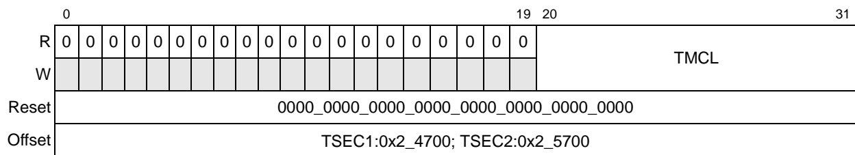
Figure 13-81. Transmit Multiple Collision Packet Counter Register Definition
