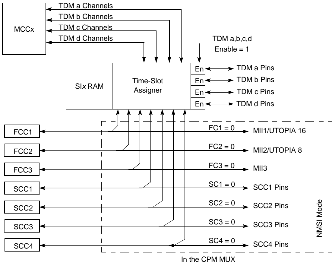
Figure 22-4. Enabling Connections to the TSA
