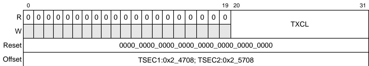
Figure 13-83. Transmit Excessive Collision Packet Counter Register Definition
