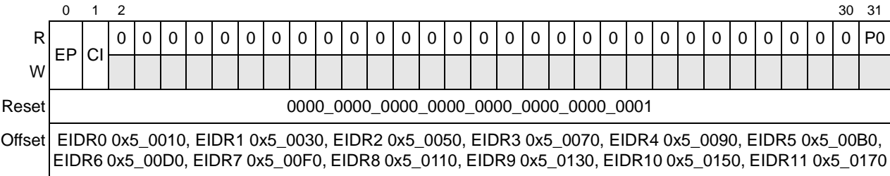
Figure 10-26. External Interrupt Destination Registers (EIDR n )
